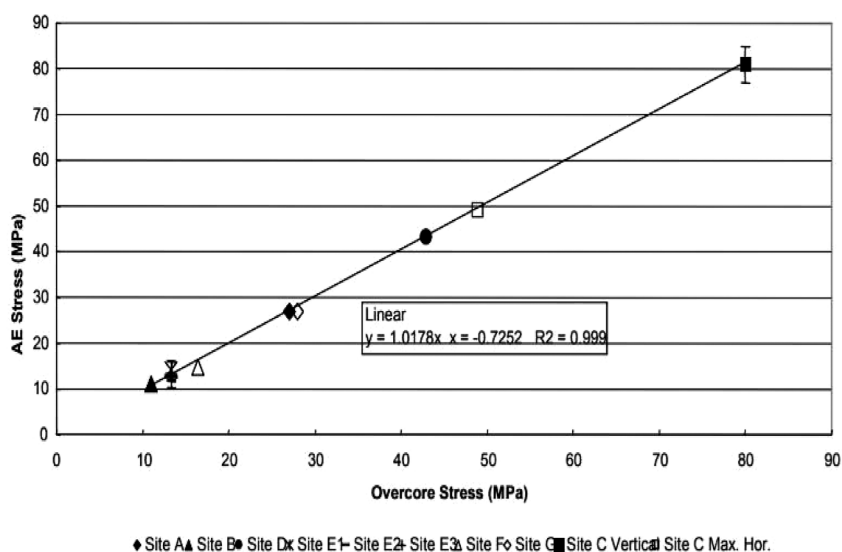
Figure 8: Comparison of stress determination from overcore stress measurement sites and AE testing for the Kaiser effect (Kent et al., 2002)
