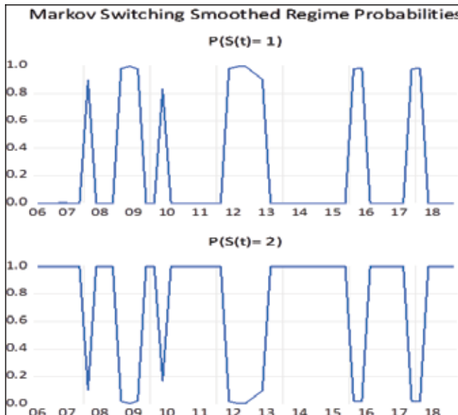
Fig. 1: Regime Probabilities
