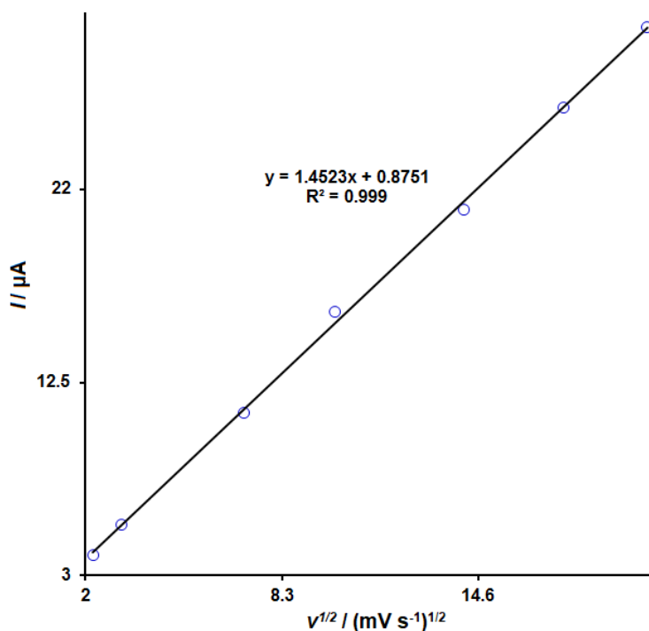
Figure 4. Plot of anodic peak current vs. v^{1/2} at different scan rates in the range of 5 to 400 mV/s
