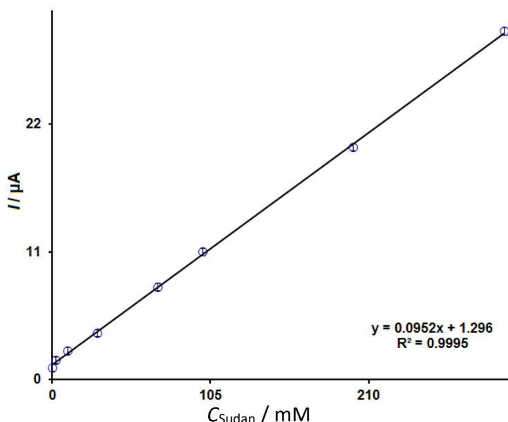
Figure 8. Plot of the electrocatalytic peak current as a function of C_{\text{Sudan}} in the range of 0.25-300.0 \mu\text{M}
