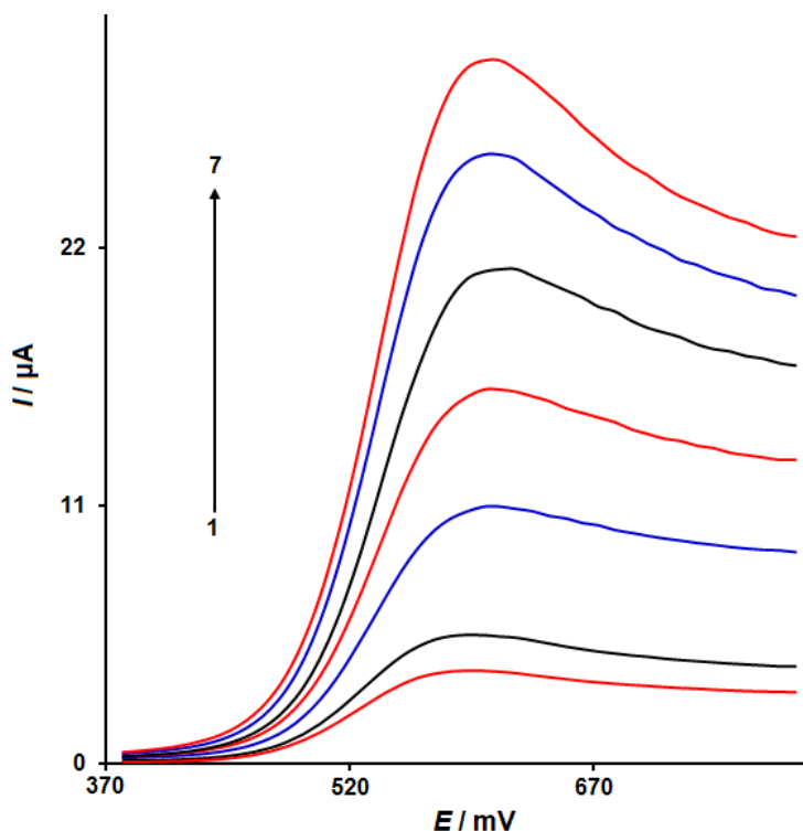
Figure 3. Linear sweep voltammograms of MnO 2 -NRs/SPE in 0.1 M PBS (pH 7.0) containing 100.0 μM Sudan at various scan rates; 1-7 correspond to 5, 10, 50, 100, 200, 300 and 400 mV s -1
