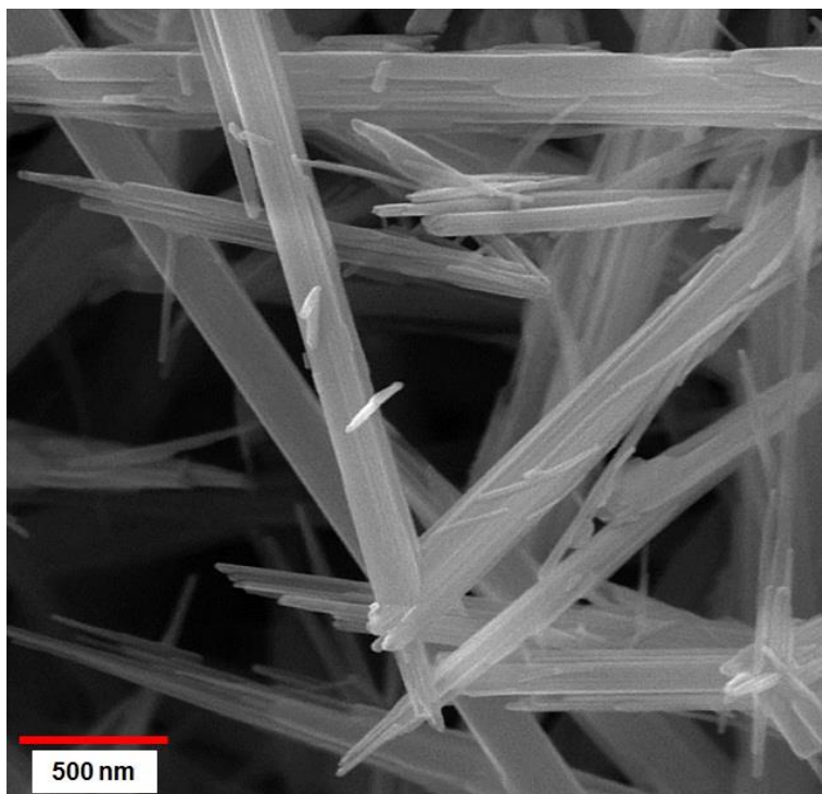
Figure 1. FE-SEM image of MnO 2 -NRs
