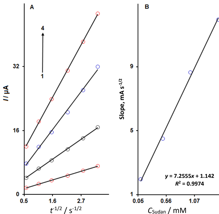
Figure 6. (A) Plots of I vs. t^{-1/2} obtained from chronoamperograms 1-4. (B) Plot of the slope of the straight lines against Sudan concentration (0.1-1.5 mM)
