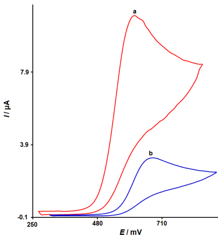
Figure 2. Cyclic voltammograms of (a) MnO 2 -NRs/SPE and (b) bare SPE in 0.1 M PBS (pH 7.0) in the presence of 100.0 \mu\text{M} Sudan at the scan rate 50 \text{ mVs}^{-1}
