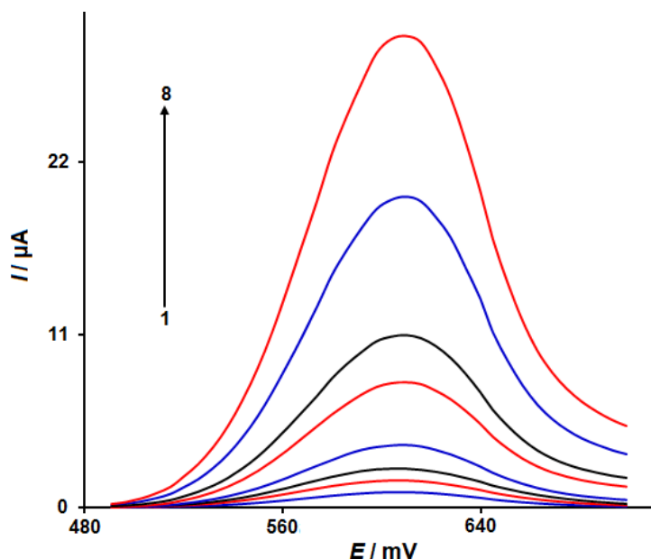
Figure 7. DPVs of \text{MnO}_2\text{-NRs/SPE} in 0.1 M (pH 7.0) containing different concentrations of Sudan. Numbers 1-8 correspond to 0.25, 2.5, 10.0, 30.0, 70.0, 100.0, 200.0 and 300.0 \mu\text{M} of Sudan
