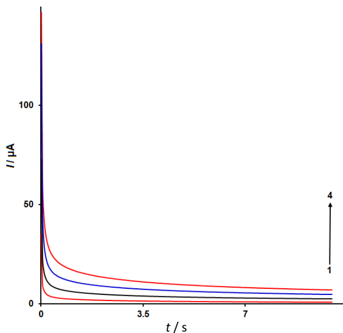
Figure 5. Chronoamperograms obtained at MnO 2 -NRs/SPE in 0.1 M PBS (pH 7.0) for different concentrations of Sudan. The 1-4 correspond to 0.1, 0.5, 1.0 and 1.5 mM of Sudan
