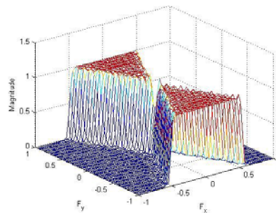
Slika 7. 2-D fan filter reda 51 i kuta 25° (metoda fwind1 ) Figure 7. 2-D fan filter of order 51, and angle 25° ( fwind1 method)
