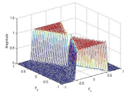
Slika 8. 2-D fan filter reda 51 i kuta 25° (metoda fwind2 ) Figure 8. 2-D fan filter of order 51, and angle 25° ( fwind2 method)
