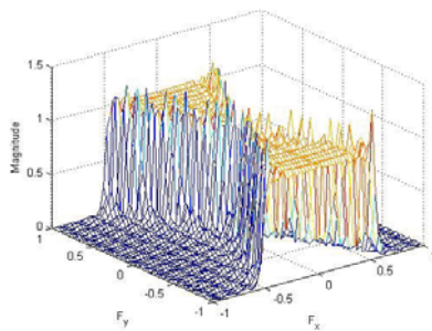
Slika 6. 2-D fan filter reda 51 i kuta 25° (metoda fsamp2 ) Figure 6. 2-D fan filter of order 51, and angle 25° ( fsamp2 method)
