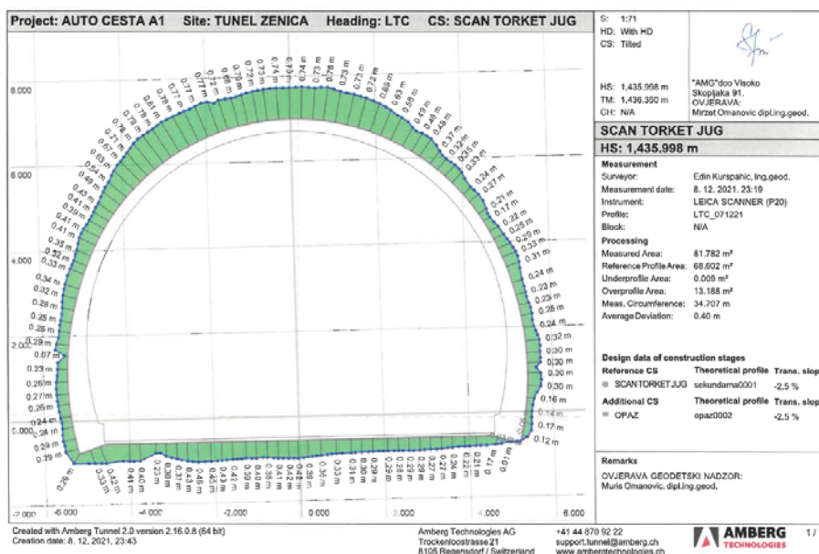
Figure 5. Geodetic survey after excavation by blasting in a weaker rock mass
