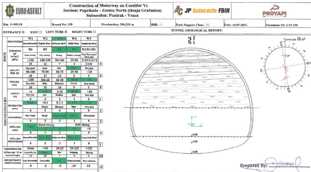
Figure 3. Geological report, chainage 1+499.10 - left tunnel tube
