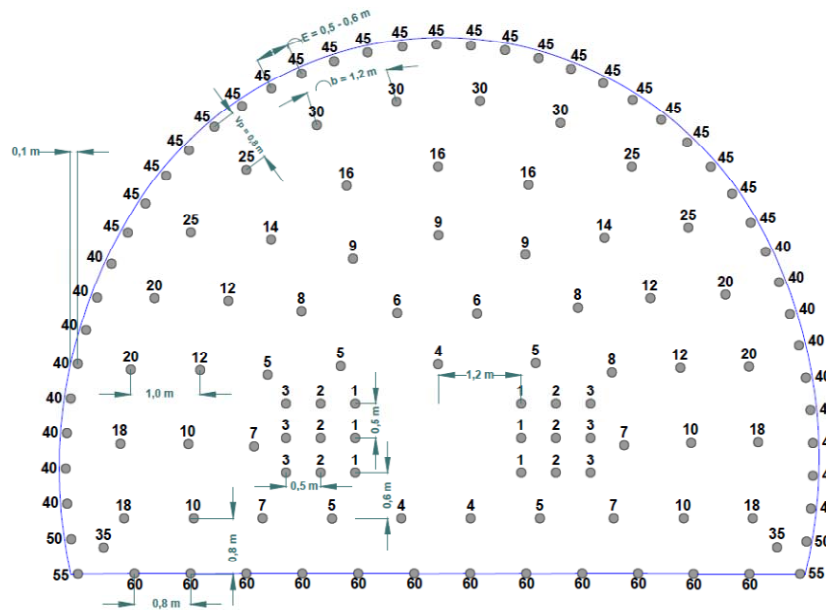
Figure 4. Layout scheme of blast holes on the cross section, as well as the layout of detonators by boreholes, for an advancement step of 3.0 m [1]
