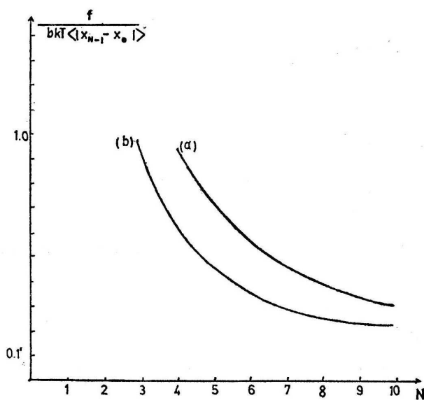
Fig. 2. a) The tension f as a function of the number N of molecular units of the macromolecular chain in the case when there exist junction points, b) The tension f as a function of the number N of molecular units of the macromolecular chain when no junction points exist.
