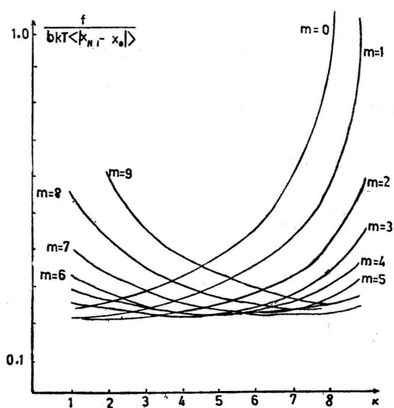
Fig. 1. The tension f as a function of K , where K is the molecule of one chain that is jointed together with the m -th molecule of the other chain ( m = 0, 1, \dots, 9 ).
