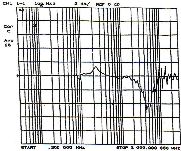
Fig. 4. Return loss measurement of the device.
