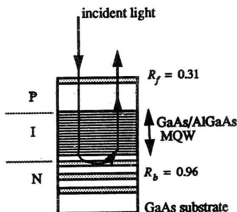
Fig. 1. Schematic cross section of the ASFP reflection modulator with front mirror reflectivity (semiconductor – air interface) R_f = 0.31 , and back mirrors reflectivity (dielectric stacks) R_b = 0.96 .
