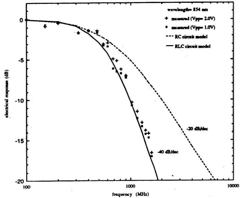
Fig. 5. Measured and calculated frequency response of the modulator.
