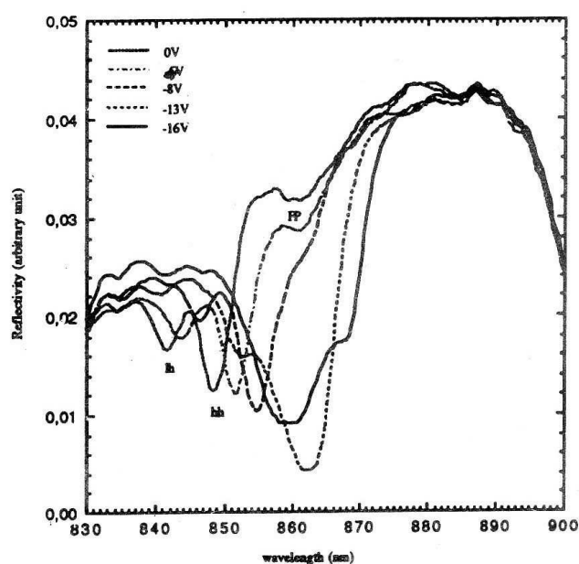
Fig. 2. Reflectivity spectra at different reverse biases.
