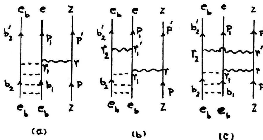
Fig. 1. Feynman diagram for ionization excitation of He by projectiles of charge Z . e_b and e represent bound and free electrons, respectively.
