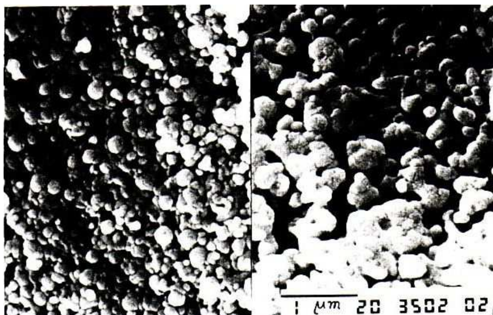
Fig. 2a. SEM of cross section of NiZ5 sample (40.39vol % of Ni).
