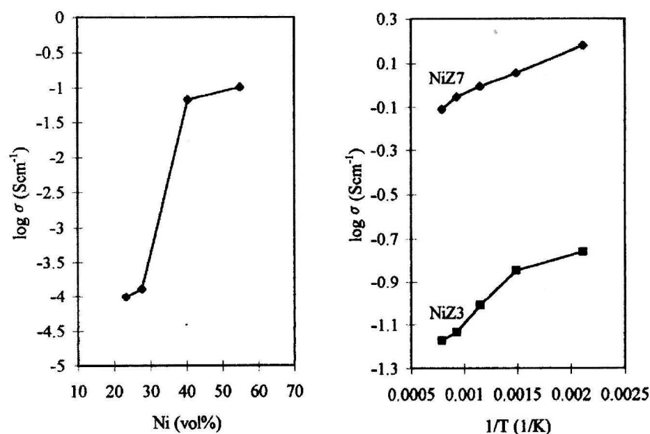
Fig. 5. Effect of Ni content on specific electrical conductivity of Ni-ZrO 2 cermets at 1000 °C.
