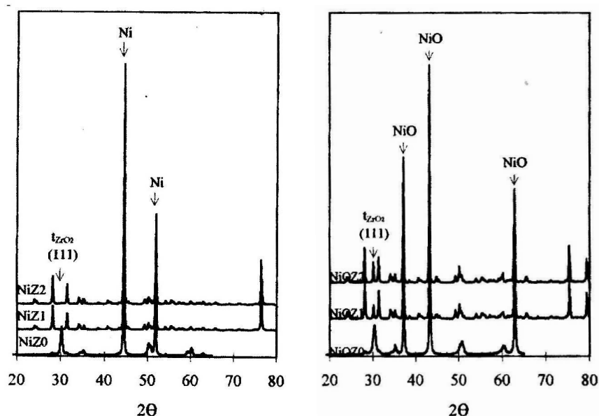
Fig. 3. X-ray diffraction patterns of NiZ samples.
