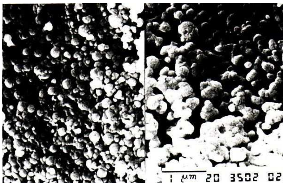
Fig. 1a. SEM of surface of NiZ5 sample (40.39vol % of Ni)
