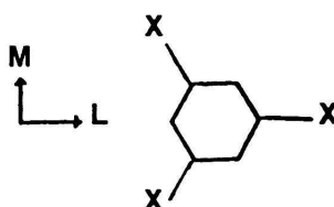
Fig.1. Structural formula of C_6H_3X_3 ( X = Cl, Br ).
