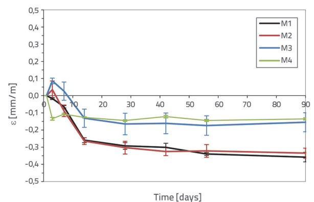
Figure 7. Autogenous shrinkage of mortars at different ages up to 90 days
