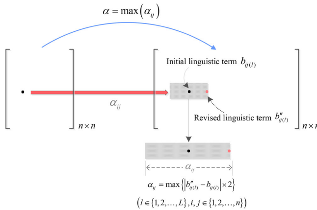
Figure 5. HFLPR with granularity level \alpha (Zheng et al., 2021c).
