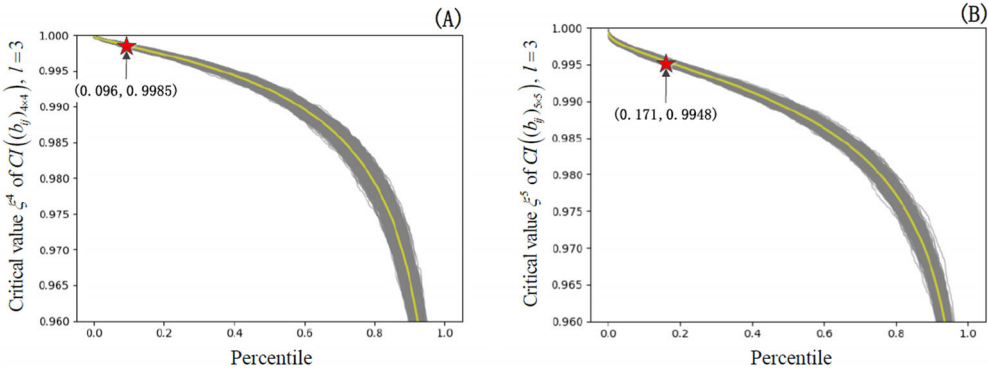
Figure 4. Thresholds \xi^4 of CI((b_{ij})_{4 \times 4}) (A) and \xi^5 of CI((b_{ij})_{5 \times 5}) (B). Source: authors' research.
