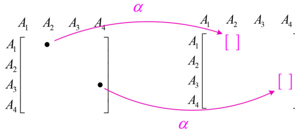
Figure 2. Information granularity in judgment matrix (Pedrycz & Song, 2011).
