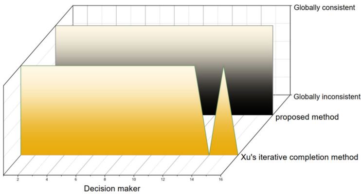
Figure 9. Whether the complete HFLPRs are globally consistent by using the proposed completion method or the Xu's iterative completion method. Source: authors' research.
