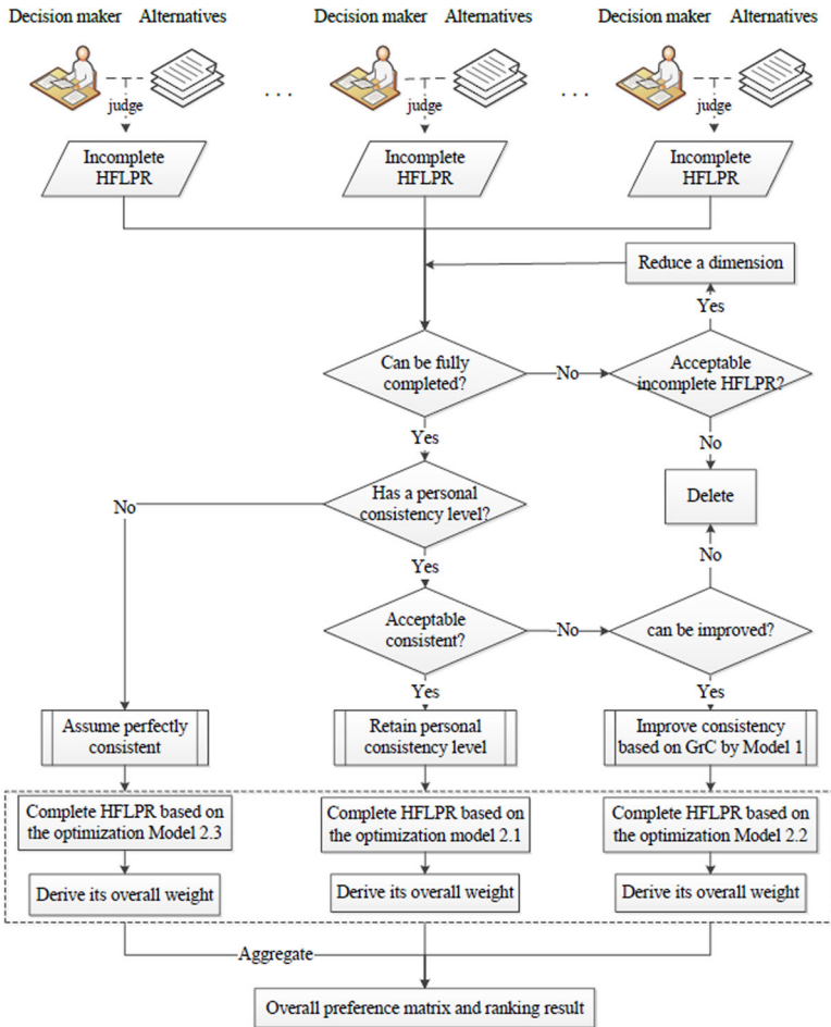
Figure 3. Framework of the proposed granular computing and optimization model-based completion method with multi-type incomplete HFLPRs for LSGDM. Source: authors' research.
