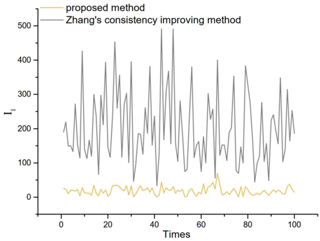
Figure 8. Different results I_1 of the proposed consistency improving method and the Zhang's consistency improving method. Source: authors' research.
