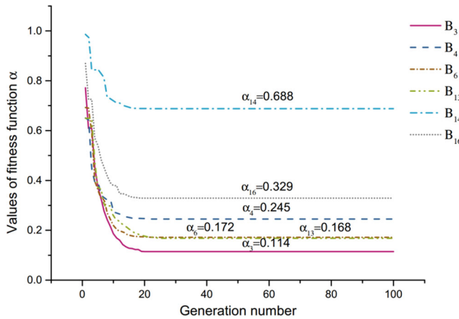
Figure 6. Values of fitness function (also granularity levels) \alpha_3, \alpha_4, \alpha_6, \alpha_{13}, \alpha_{14}, \alpha_{16} calculated by the PSO algorithm. Source: authors' research.
