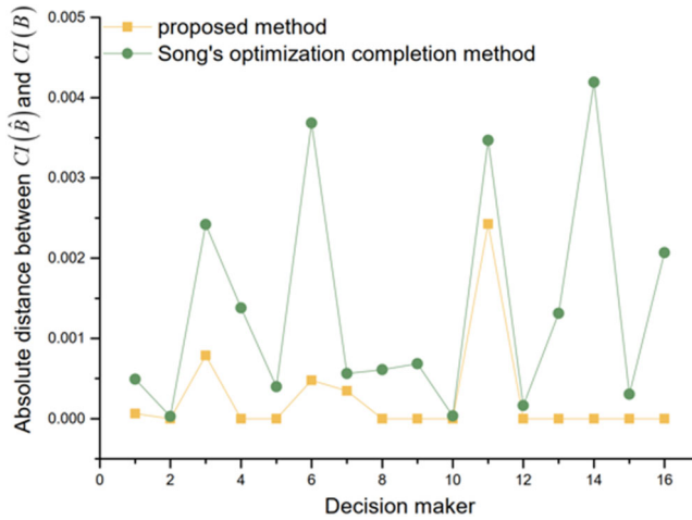
Figure 11. Absolute distance between CI(\hat{B}) and CI(B) by using the proposed completion method and the Song’s optimization completion method. Source: authors’ research.
