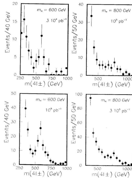
Fig. 4. The invariant mass of 4l^\pm superimposed on the ZZ background for a) m_H = 600 GeV and L = 3 \cdot 10^4 \text{ pb}^{-1} , b) m_H = 800 GeV and L = 10^5 \text{ pb}^{-1} , c) m_H = 600 GeV and L = 10^5 \text{ pb}^{-1} and d) m_H = 800 GeV and L = 3 \cdot 10^5 \text{ pb}^{-1} .
