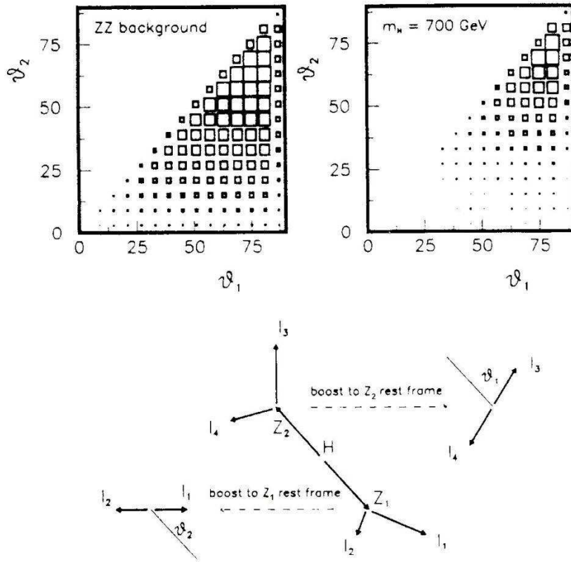
Fig. 2. Angular distributions of leptons coming from a pair of Z 's ( \vartheta_1 > \vartheta_2 ) in the Z helicity frame for the ZZ background in the interval m_{ZZ} = m_H \pm 2\sigma_H and for the signal, all for m_H = 700 GeV. Also shown is an illustration of H \rightarrow ZZ \rightarrow 4l^\pm decay in the Z helicity frame.
