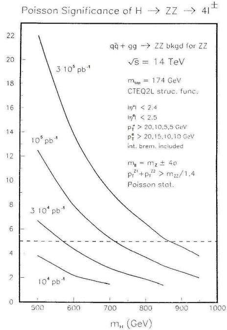
Fig. 5. The significance of the signal for different Higgs masses, calculated according to Poisson statistics and for various integrated luminosities.
