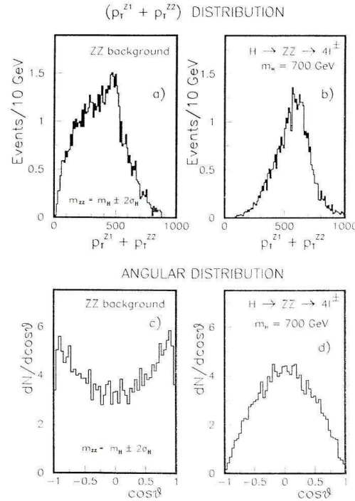
Fig. 1. a) Distribution of p_T^{Z1} + P_T^{Z2} for ZZ background in the mass window m_{ZZ} = m_H \pm 2\sigma_H for m_H = 700 GeV. b) Distribution of p_T^{Z1} + P_T^{Z2} for the Higgs signal at m_H = 700 GeV. c) Lepton angular distribution for ZZ background in the window m_{ZZ} = m_H \pm 2\sigma_H for m_H = 700 GeV. d) Angular distribution of the signal for m_H = 700 GeV.
