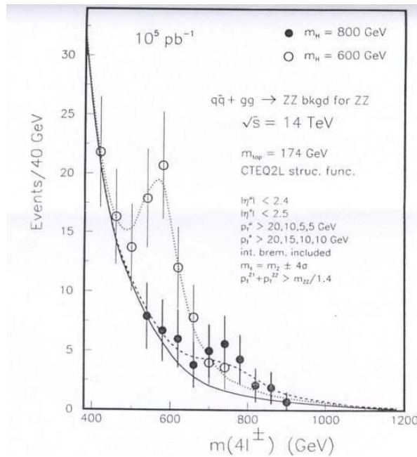
Fig. 3. The invariant mass of 4l^\pm for m_H = 600 \text{ GeV} (dotted and dashed lines, respectively) over the continuum background (full line) for an integrated luminosity of 10^5 \text{ pb}^{-1} . The circles represent the signal points with their statistical errors.
