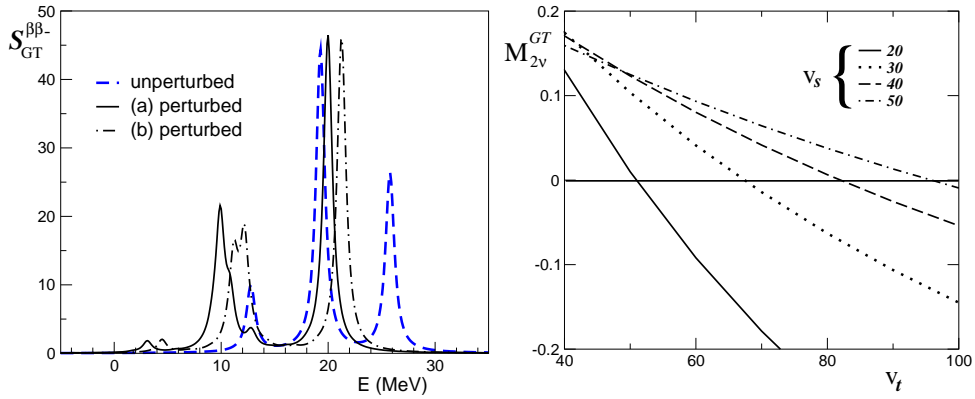
Fig. 4 (left). Graphical representation of energy dependence of the double GT strengths S_{\text{GT}}^{\beta\beta^-} , measured from the ^{48}\text{Ca} ground state. The coupling constant values in the perturbed calculations were v_s = 35 , v_t = 65 for case (a), and v_s = 40 , v_t = 60 for case (b).
