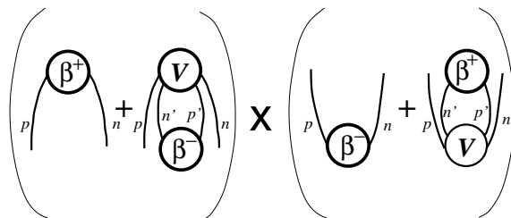
Fig. 2. Graphical representation of the numerator in (6) within the QRPA. The first and second terms match, respectively, to \langle \tilde{1}_{\alpha}^{+} || \mathcal{O}_1^{\beta^{+}} || \tilde{0}^{+} \rangle and \langle \tilde{1}_{\alpha}^{+} || \mathcal{O}_1^{\beta^{-}} || \tilde{0}^{+} \rangle , given by (33). The vertices \beta^{\pm} stand for \tilde{\Lambda}_{\pm}^{0}(pn) , while the residual interaction brings about the ground-state correlations in the vertex V .
