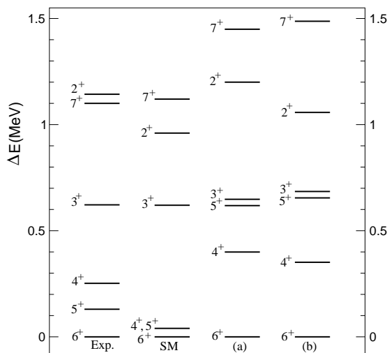
Fig. 6. Comparison between the experimental and theoretical energy levels of ^{48}\text{Sc} for the cases (a) v_s = 35 , v_t = 65 , and (b) v_s = 40 , v_t = 60 . We also display the shell-model results from Ref. [71].
