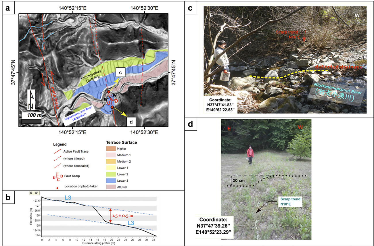
Figure 8: (a) The distribution of terrace surfaces and active fault trace along the Migisasookoizumi River in Yamagadaira site overlaid on 2-m slope map; (b) Topographic profile B – B' across the fault trace; (c) Deflected drainage river bed; (d) Subtle fault scarp in L3 terrace.
