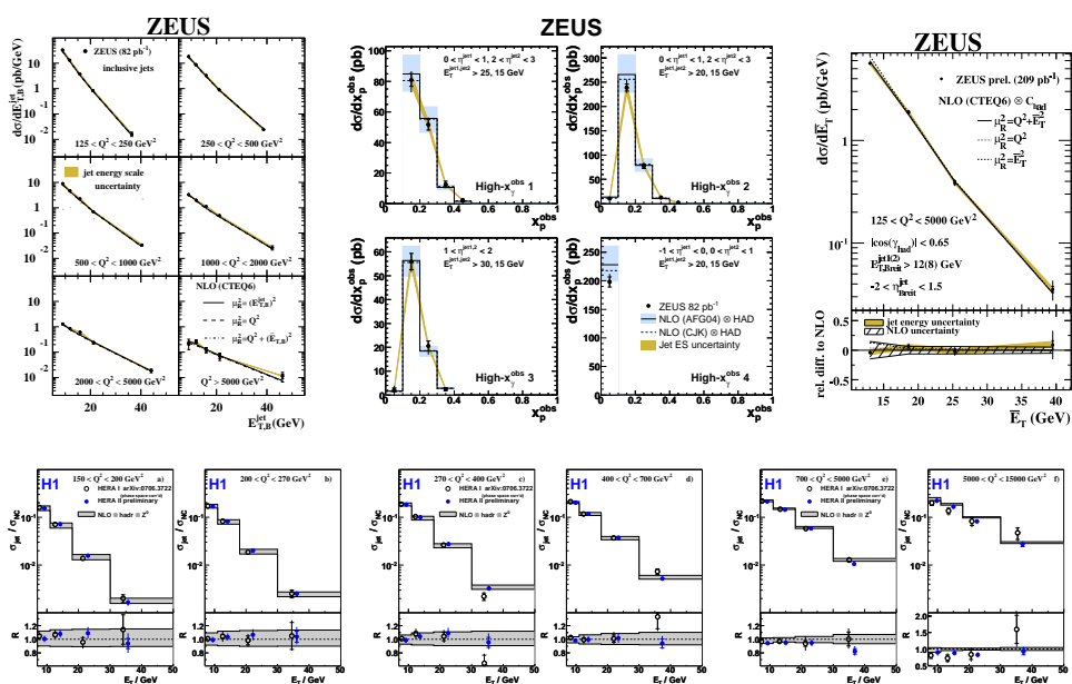
Fig. 9. Upper plots: ZEUS jet data from; (left) inclusive DIS (HERA-I, 82 \text{ pb}^{-1} ), (middle) di-jet photoproduction (HERA-I, 82 \text{ pb}^{-1} ), (right) di-jet DIS (HERA-II, 209 \text{ pb}^{-1} ). Lower plots: H1 normalised inclusive jet cross-sections (HERA-I and HERA-II, 320 \text{ pb}^{-1} ).
