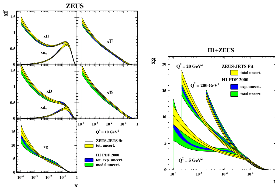
Fig. 2. Left: Comparison of PDFs from ZEUS and H1 analyses at Q^2 = 10 \text{ GeV}^2 . Right: Comparison of gluon from ZEUS and H1 analyses, at various Q^2 . Note that the ZEUS analysis total uncertainty includes both experimental and model uncertainties.
