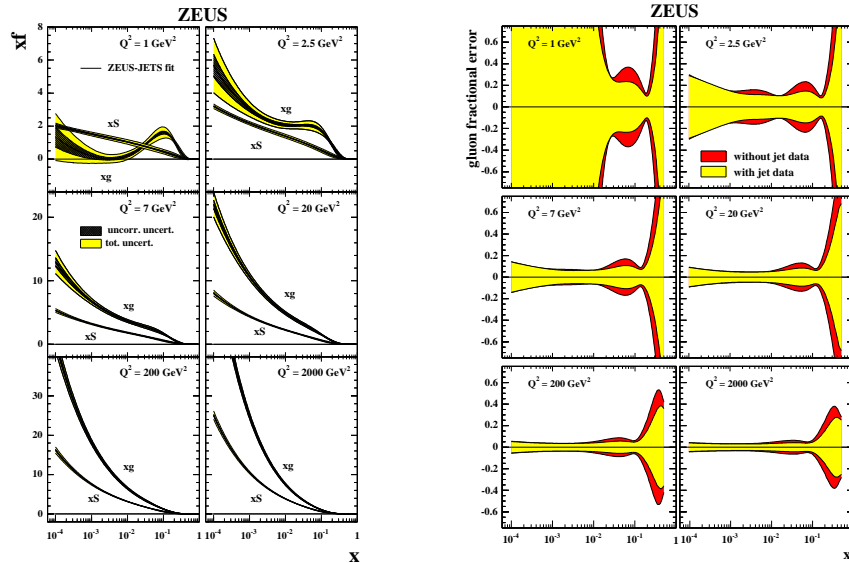
Fig. 4. Left: the sea and gluon PDFs from the ZEUS-JETS fit for various Q^2 values. Right: The fractional error on the gluon PDF for various Q^2 values, for PDF fits made with and without including the jet data.
