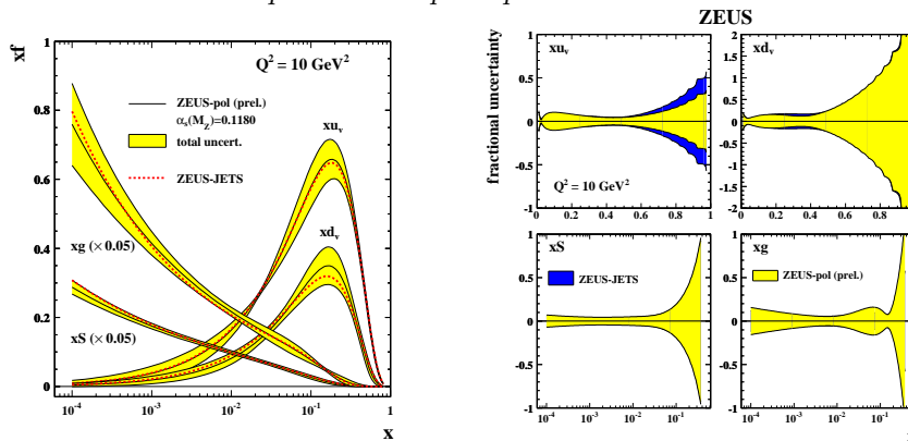
Fig. 8. Left: The PDFs extracted from the ZEUS-pol fit and their uncertainties, compared to the ZEUS-JETS fit at Q^2 = 10 \text{ GeV}^2 . Right: The fractional uncertainties of the ZEUS-pol PDFs compared to those of the ZEUS-JETS PDFs.
