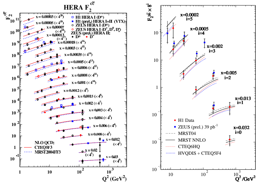
Fig. 10. Heavy quark production data compared to predictions from different PDF sets using different heavy quark production schemes. Left: F_2^{c\bar{c}} data from HERA. Right: F_2^{b\bar{b}} data from HERA.
