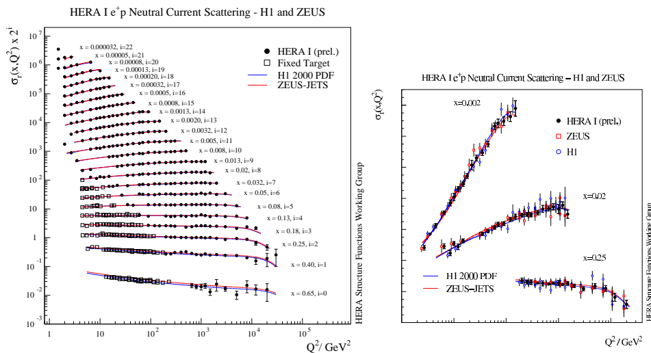
Fig. 3. Left: HERA-I combined data on \sigma_r as a function of Q^2 for NC e^+p scattering, together with fixed target data, for x bins across the whole measured kinematic plane. Right: H1, ZEUS and HERA-I combined data on \sigma_r for NC e^+p scattering for low, middling and high- x .
