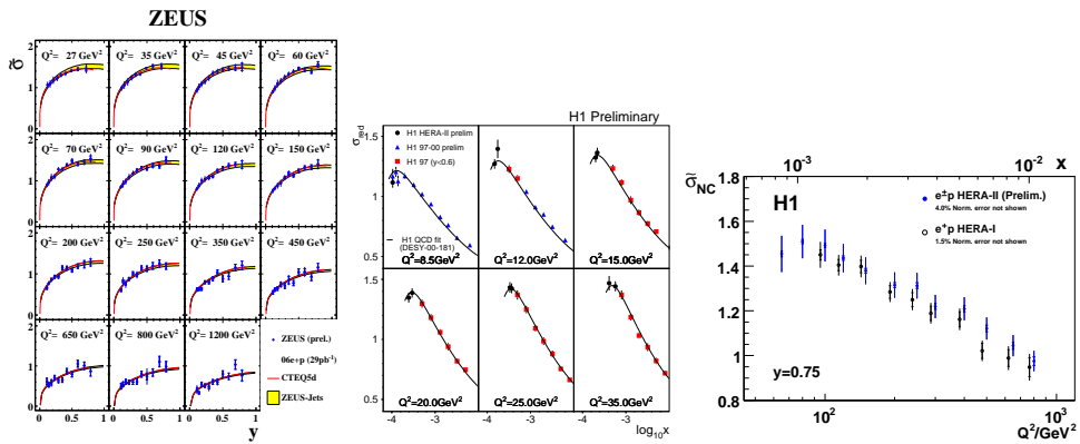
Fig. 11. HERA data at high y from: (left) ZEUS HERA-II, (middle) H1 HERA-I at low Q^2 and (right) H1 HERA-II at high- Q^2 .
