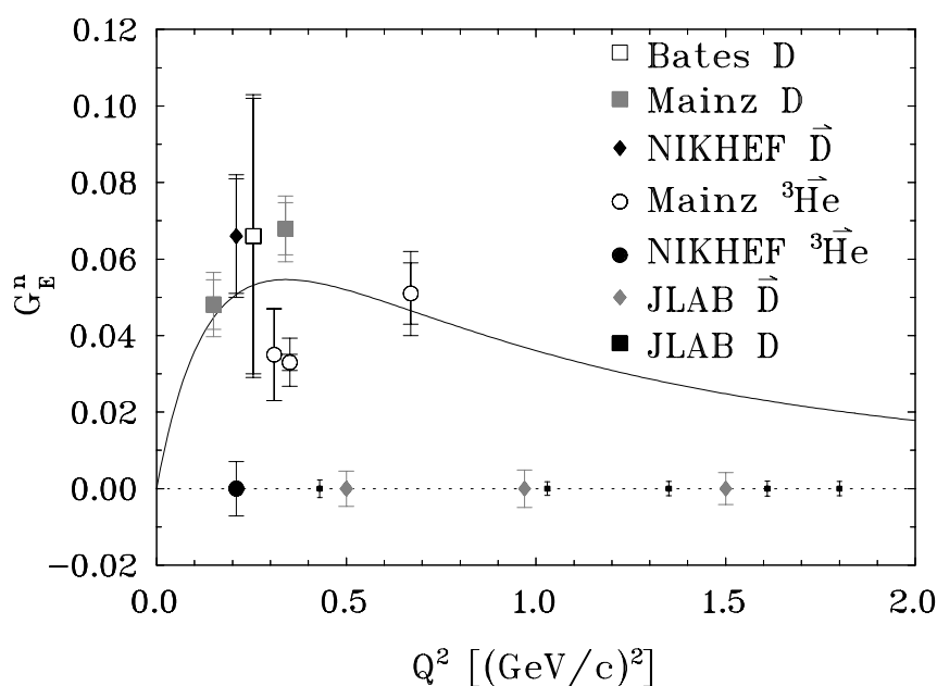
Fig. 1. The electric form-factor of the neutron G_E^n as a function of Q^2 . The parameterization is from the work of Galster et al., where G_E^n = -\tau\mu_n G_D(1 + 5.6\tau)^{-1} . See text for explanation of points.
