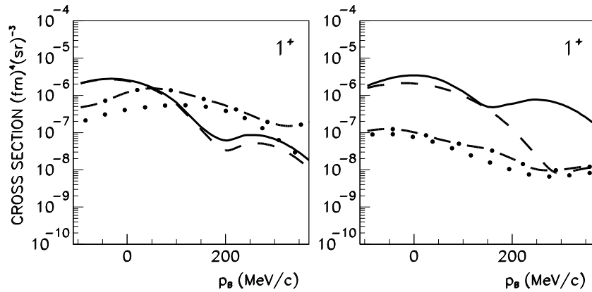
Fig. 4. The differential cross section of the ^{16}\text{O}(e,e'pn) reaction to the 1^+ ground state of ^{14}\text{N} in the same superparallel kinematics as in Fig. 2. Line convention in the left panel: DW with the \Delta -current (dotted), DW-NN with the \Delta -current (dash-dotted), DW with the one-body-part (dashed), DW-NN with the one-body-part (solid). Line convention in the right panel: DW with the pion-in-flight-current (dotted), DW-NN with the pion-in-flight-current (dash-dotted), DW with the seagull-current (dashed), DW-NN with the seagull-current (solid).
