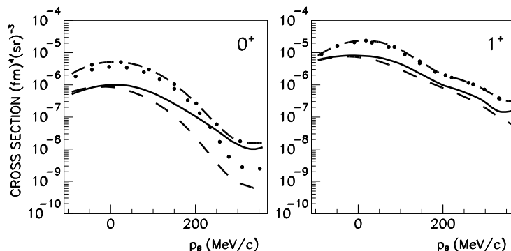
Fig. 2. The differential cross section of the ^{16}\text{O}(e,e'\text{pp}) reaction to the 0^+ ground state of ^{14}\text{C} (left panel) and of the ^{16}\text{O}(e,e'\text{pn}) reaction to the 1^+ ground state of ^{14}\text{N} (right panel) in superparallel kinematics with an incident electron energy E_0 = 855 MeV, an electron scattering angle \theta_e = 18^\circ , energy transfer \omega = 215 MeV and q = 316 MeV/c. In ^{16}\text{O}(e,e'\text{pn}) the proton is ejected parallel and the neutron antiparallel to \mathbf{q} . Different values of p_B are obtained changing the kinetic energies of the outgoing nucleons. Positive (negative) values of p_B refer to situations where \mathbf{p}_B is parallel (anti-parallel) to \mathbf{q} . Line convention: PW (dotted), PW-NN (dash-dotted), DW (dashed), DW-NN (solid).
