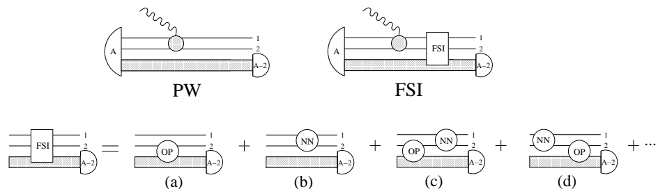
Fig. 1. The relevant diagrams for electromagnetic two-nucleon knockout on a complex nucleus. The two diagrams on top depict the plane-wave approximation (PW) and the distortion of the two outgoing proton wave functions by the final state interaction (FSI). Below, the relevant mechanisms of FSI are depicted in detail, where the open circle denotes either a nucleon-nucleus interaction given by a phenomenological optical potential (OP) or the mutual interaction between the two outgoing nucleons (NN). Diagrams which are given by an interchange of nucleon 1 and 2 are not depicted.
