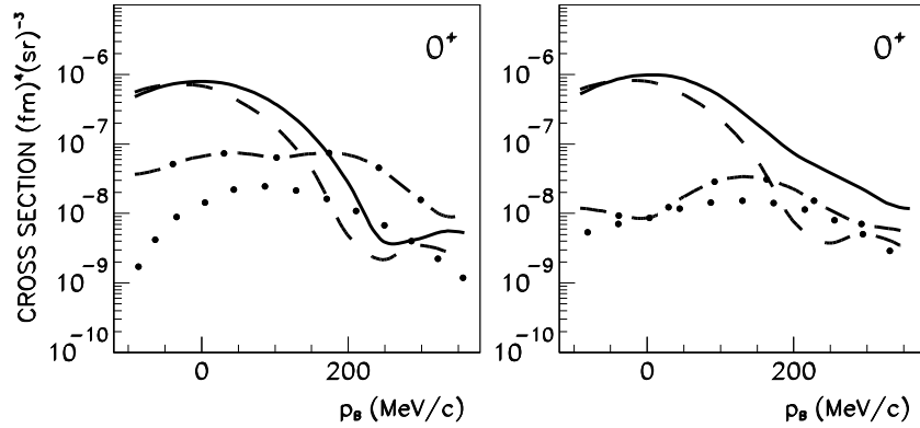
Fig. 3. The differential cross section of the ^{16}\text{O}(e,e'pp) reaction to the 0^+ ground state of ^{14}\text{C} in the same superparallel kinematics as in Fig. 2. Line convention for the left panel: DW with the \Delta -current (dotted), DW-NN with the \Delta -current (dash-dotted), DW with the one-body current (dashed), DW-NN with the one-body current (solid). In the right panel the dashed (solid) curve shows the separate contribution of the ^1S_0 relative partial wave in a DW (DW-NN) calculation. The dotted (dash-dotted) curve shows the separate contribution of the ^3P_1 relative partial wave in a DW (DW-NN) calculation.
