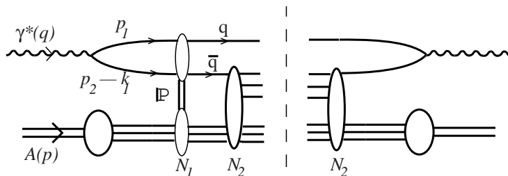
Fig. 5. Glauber-Gribov shadowing involves interference between rescattering amplitudes. .
