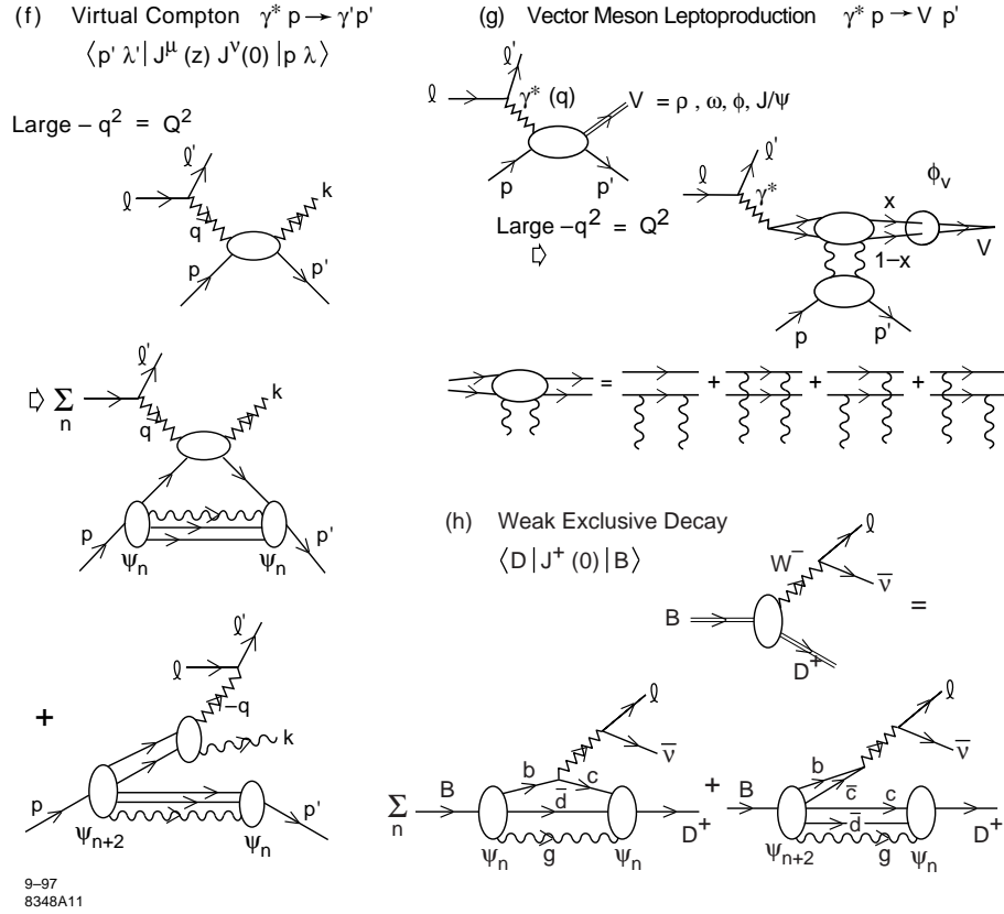
Fig. 2. (f) Representation of deeply virtual Compton scattering in the light-cone Fock expansion in the handbag approximation and at leading twist. Both diagonal n \rightarrow n and off-diagonal n + 2 \rightarrow n contributions are required. (g) Diffractive vector meson production at large photon virtuality Q^2 and longitudinal polarization. The high energy behavior involves two gluons in the t channel coupling to the compact color dipole structure of the upper vertex. The bound-state structure of the vector meson enters through its distribution amplitude. (h) Exact representation of the weak semileptonic decays of heavy hadrons in the light-cone Fock expansion. Both diagonal n \rightarrow n and off-diagonal pair annihilation n + 2 \rightarrow n contributions are required.
