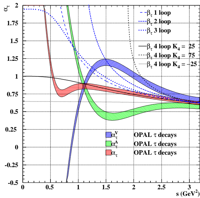
Fig. 3. The effective charge \alpha_\tau for non-strange hadronic decays of a hypothetical \tau lepton with m_{\tau'}^2 = s compared to solutions of the fixed order evolution equation for \alpha_\tau at two-, three-, and four-loop order. The error bands include statistical and systematic errors.
