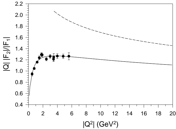
Fig. 4. Perturbative QCD motivated fit to the Jefferson Lab polarization transfer data [77, 78]. The parametrization is given in Eq. (5) of the text. The dashed line shows the predicted form for timelike q^2 = -Q^2 . For a discussion on the validity of continuing spacelike form factors to the timelike region, see [79]
