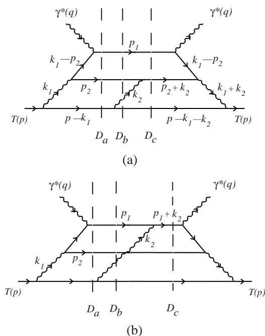
Fig. 6. Two types of final state interactions. (a) Scattering of the antiquark ( p_2 line), which in the aligned jet kinematics is part of the target dynamics. (b) Scattering of the current quark ( p_1 line). For each LC time-ordered diagram, the potentially on-shell intermediate states—corresponding to the zeroes of the denominators D_a, D_b, D_c —are denoted by dashed lines.
