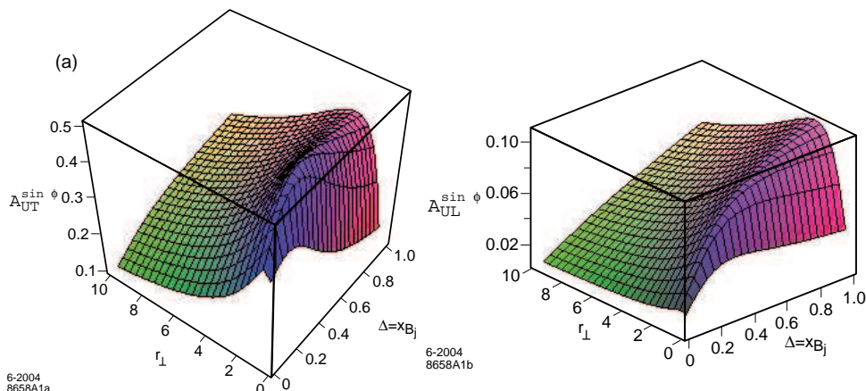
Fig. 7. Model predictions for the target single-spin asymmetry A_{UT}^{\sin\phi} for charged and neutral current deep inelastic scattering resulting from gluon exchange in the final state. Here r_{\perp} is the magnitude of the transverse momentum of the outgoing quark relative to the photon or vector boson direction, and \Delta = x_{bj} is the light-cone momentum fraction of the struck quark. The parameters of the model are given in the text. In (a) the target polarization is transverse to the incident lepton direction. The asymmetry in (b) A_{UL}^{\sin\phi} = K A_{UT}^{\sin\phi} includes a kinematic factor K = \frac{Q}{\nu} \sqrt{1-y} for the case where the target nucleon is polarized along the incident lepton direction. For illustration, we have taken K = 0.26\sqrt{x} , corresponding to the kinematics of the HERMES experiment [116] with E_{lab} = 27.6 GeV and y = 0.5 .
