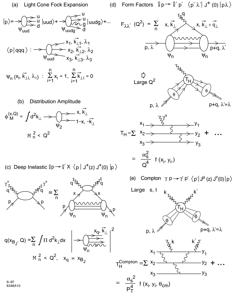
Fig. 1. Representation of QCD hadronic processes in the light-cone Fock expansion. (a) The valence uud and uudg contributions to the light-cone Fock expansion for the proton. (b) The distribution amplitude \phi(x, Q) of a meson expressed as an integral over its valence light-cone wave function restricted to q\bar{q} invariant mass less than Q . (c) Representation of deep inelastic scattering and the quark distributions q(x, Q) as probabilistic measures of the light-cone Fock wave functions. The sum is over the Fock states with invariant mass less than Q . (d) Exact representation of spacelike form factors of the proton in the light-cone Fock basis. The sum is over all Fock components. At large momentum transfer the leading-twist contribution factorizes as the product of the hard scattering amplitude T_H for the scattering of the valence quarks collinear with the initial to final direction convoluted with the proton distribution amplitude. (e) Leading-twist factorization of the Compton amplitude at large momentum transfer.
