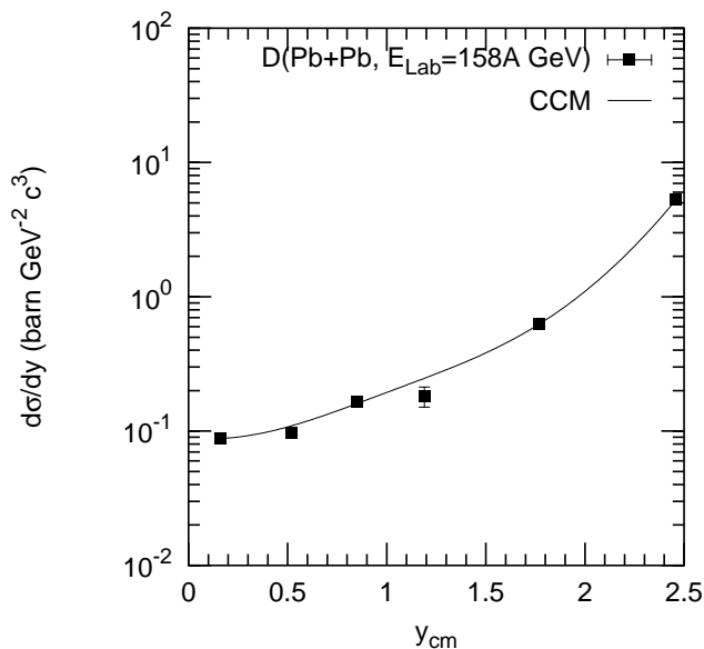
Fig. 3. Rapidity spectra for production of secondary deuterons in PbPb collisions at an energy E_{\text{lab}} = 158A GeV. The experimental data are taken from Ref. [18] while the solid curve is on the basis of CCM.
