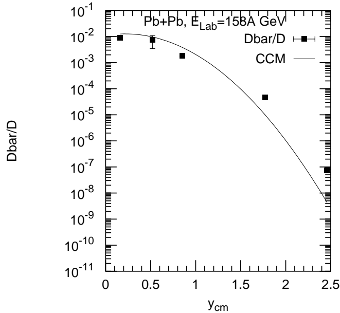
Fig. 5. Nature of \bar{D}/D ratio as a function of c.m. rapidity. The experimental data are for PbPb collisions at E_{lab} = 158A GeV [18]. The solid curvilinear line depicts the CCM-based results.
