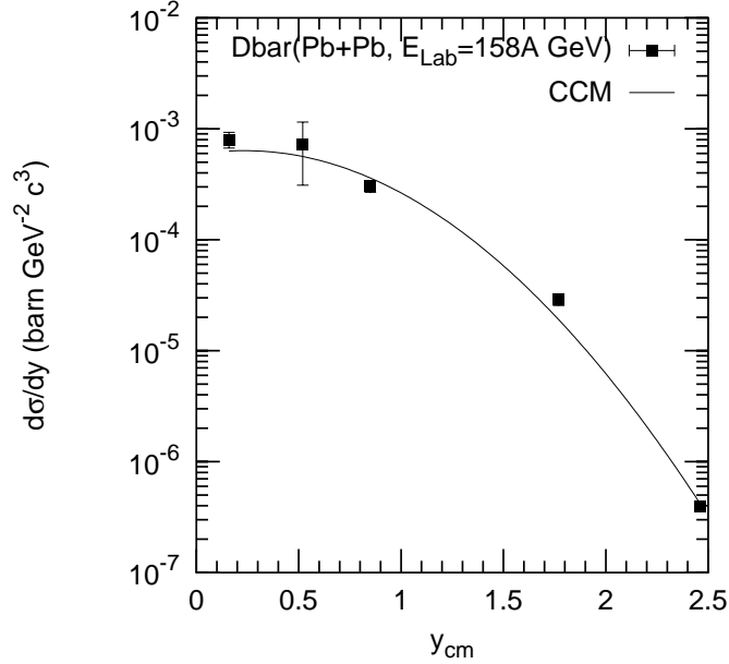
Fig. 4. Rapidity spectra for production of secondary antideuterons in PbPb collisions at an energy E_{lab} = 158A GeV. The experimental data are taken from Ref. [18] while the solid curve is on the basis of CCM.
