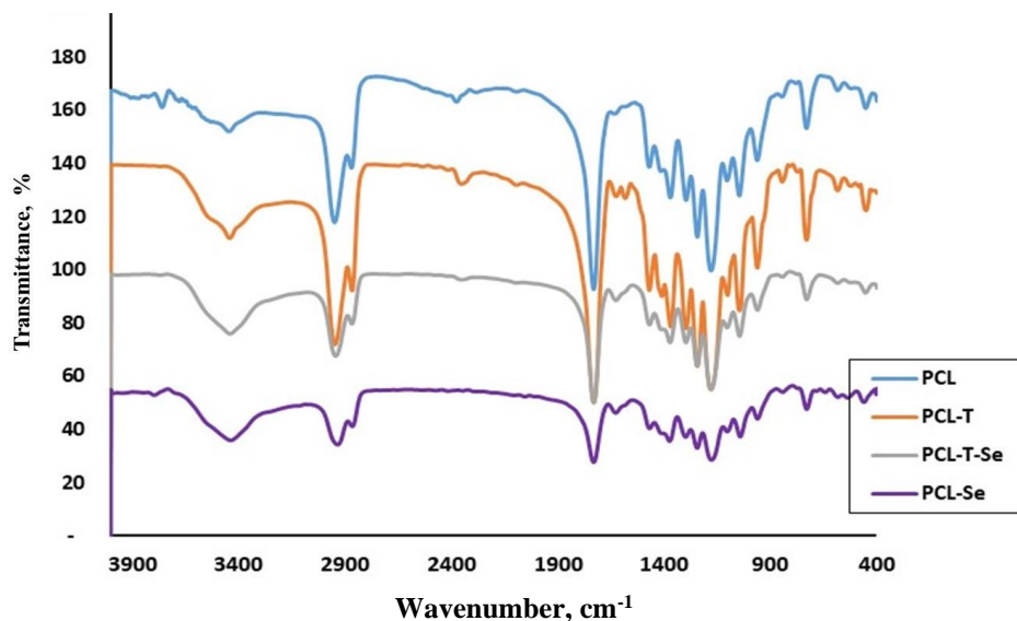
Figure 3. FTIR of PCL, PCL-triazole, PCL-triazole-Se and PCL-Se nanoparticles.
