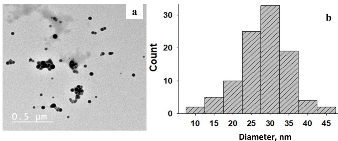
Figure 2. TEM of SeNPs and their diameter distribution histogram from image analysis.
