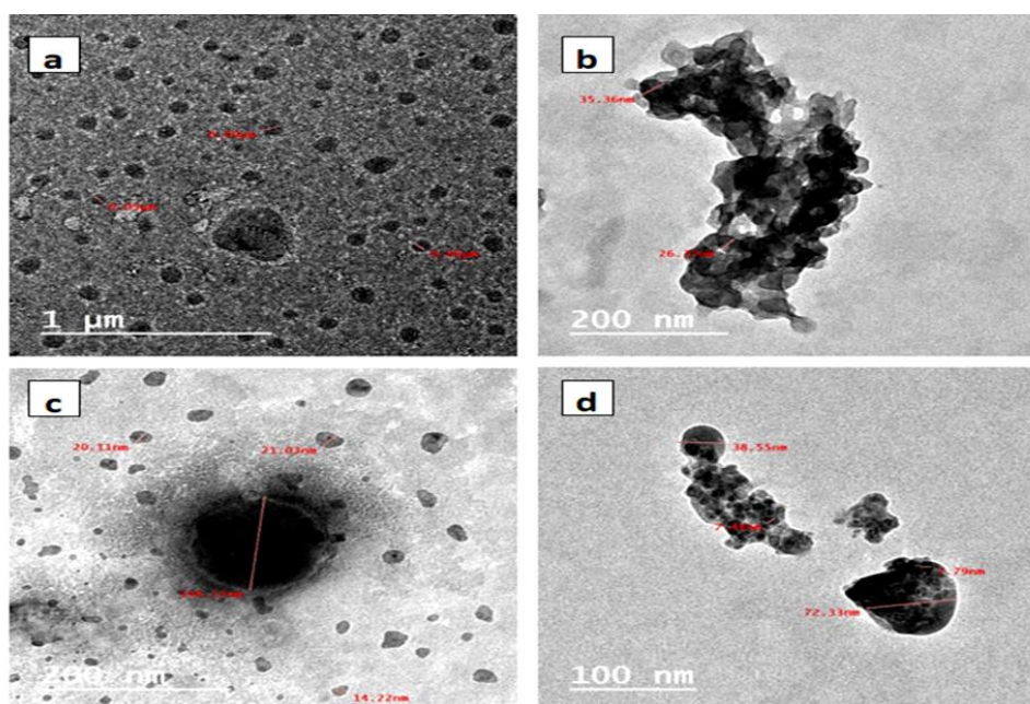
Figure 4. TEM of (a) PCL, (b) PCL-triazole, (c) PCL-triazole- Se and (d) PCL-Se nanoparticles.
