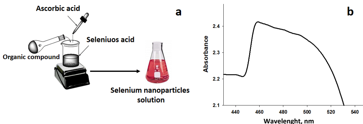
Figure 1. (a) The pathway for the synthesis of SeNPs, (b) UV-Vis spectrum of SeNPs.
