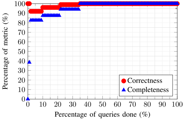
Fig. 6. An example of a run where 3 counterexamples were found.
