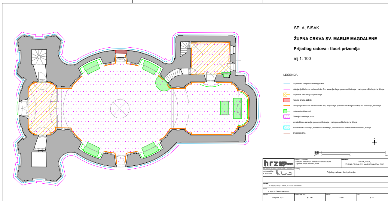
17 Crkva sv. Marije Magdalene u Selima, prijedlog radova – tlocrt prizemlja (crtali: T. Prpić, A. Škevin Mikulandra, dokumentacija HRZ, 2022.) Church of St. Mary Magdalene in Sela, proposal for works – floor plan of the ground floor (drawings: T. Prpić, A. Škevin Mikulandra, Croatian Conservation Institute documentation, 2022)
