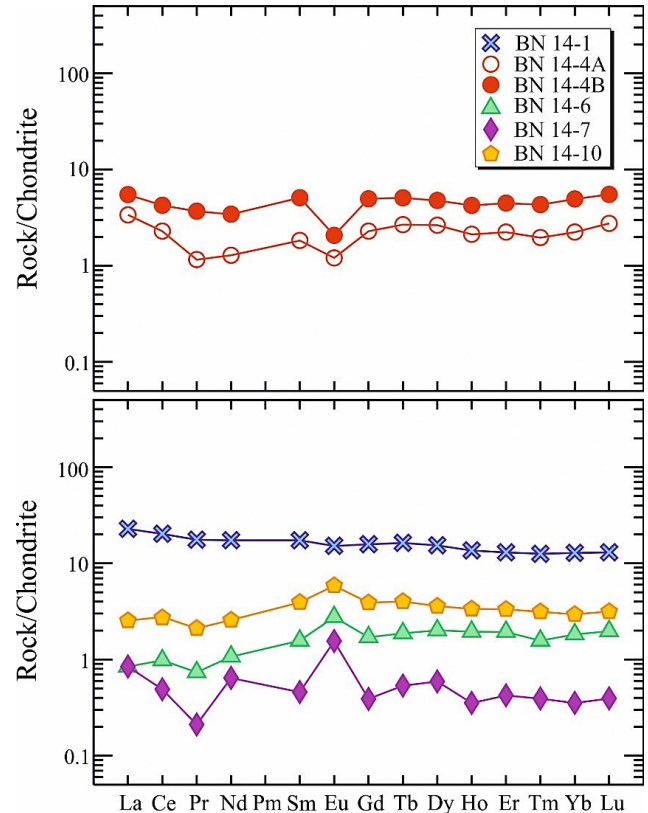
Figure 10: Chondrite normalised REE diagrams. Normalisation values are after Sun and McDonough (1989). Trace element distribution of peridotite sample BN-14B is indicated by full red circles and all other symbols represent different amphibolite samples.
