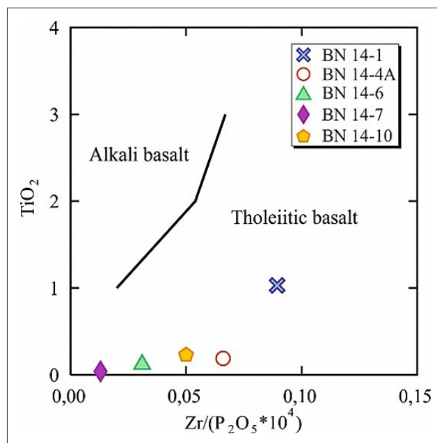
Figure 12: \text{TiO}_2\text{-Zr}/(\text{P}_2\text{O}_5 \cdot 10^4) diagram after Winchester & Floyd (1977)
