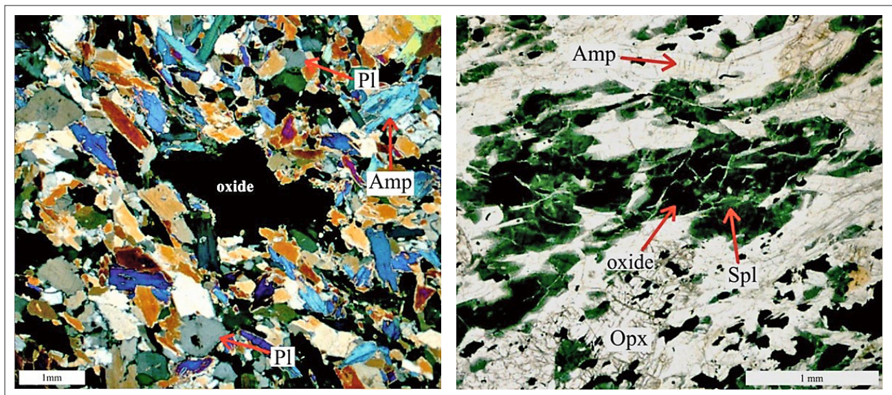
Figure 8: Left: Nematogranoblastic texture of BN 14-4A (N+). Right: Green spinel surrounding opaque oxide mineral grains in BN 14-4B (N). Amp=amphibole; Opx=orthopyroxene; Pl=plagioclase; Spl=spinel. Mineral abbreviations after Slovenec and Bermanec (2003).
