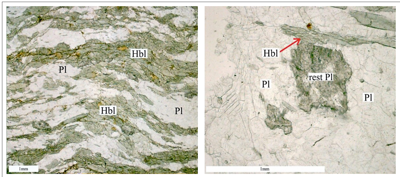
Figure 7: Left: Folding on the microscale in BN 14-10 (N). Right: Relict of the primary (magmatic) plagioclase altered to clay minerals and clinozoisite in BN 14-10 (N). Czo=clinozoisite; Hbl=hornblende; Pl=plagioclase; rest Pl=magmatic plagioclase relict. Mineral abbreviations after Slovenec and Bermanec (2003).
