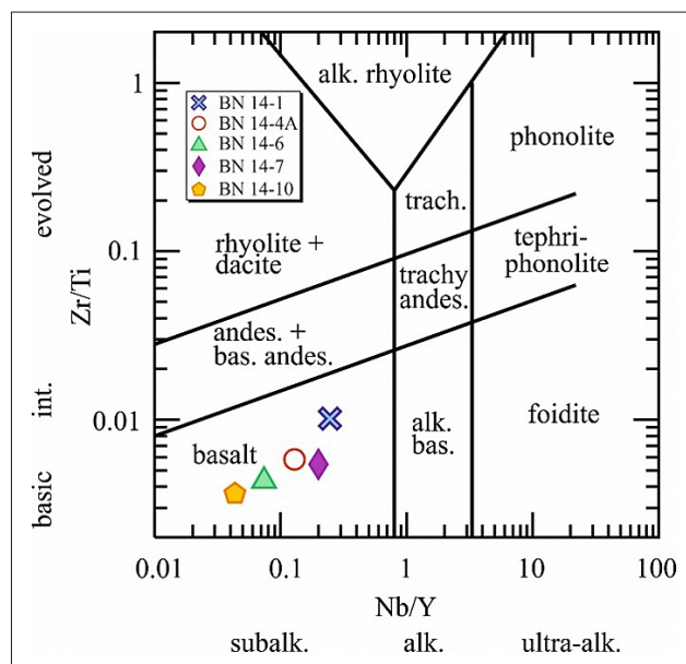
Figure 11: Zr/Ti-Nb/Y classification diagram after Pearce (1996)
