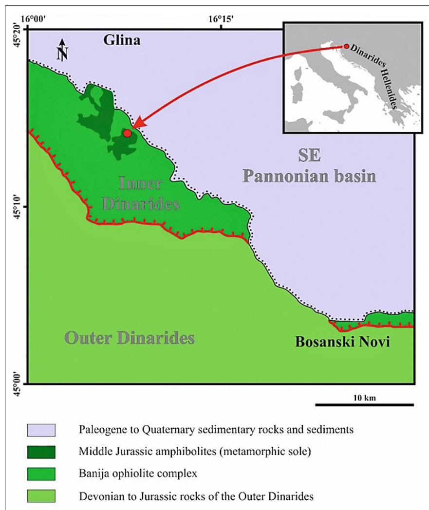
Figure 1: Schematic geological map of the investigated area after Šikić et al. (1990). Location of the Slatina Quarry from which the investigated amphibolites were taken is indicated in red.
