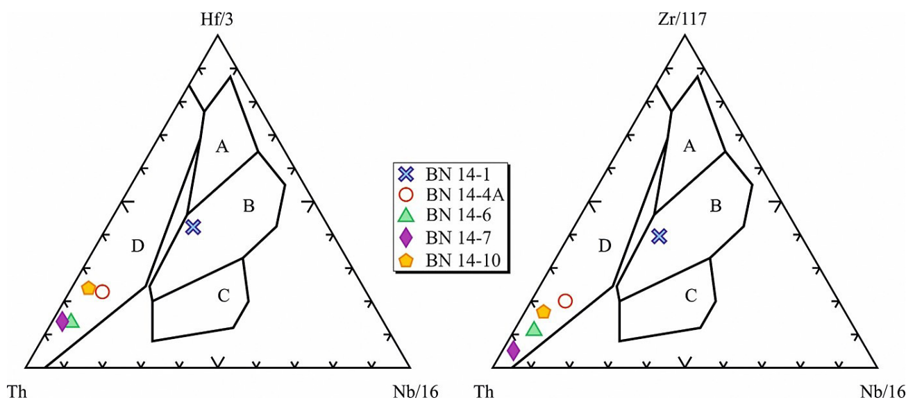
Figure 13: Th-Hf/3-Nb/16 and Th-Zr/117-Nb/16 diagrams after Wood (1980). A=N-MORB (Normal Mid-Ocean Ridge Basalt); B=E-MORB (Enriched Mid-Ocean Ridge Basalt); C=OIB (Ocean Island Basalt); D=IAT (Island Arc Tholeiite).
