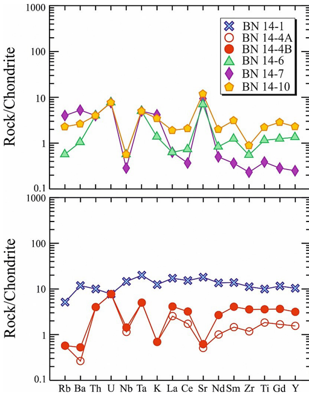
Figure 9: Chondrite normalised spider diagrams. Normalisation values are after Sun and McDonough (1989). Trace element distribution of peridotite sample BN-14B is indicated by full red circles and all other symbols represent different amphibolite samples.
