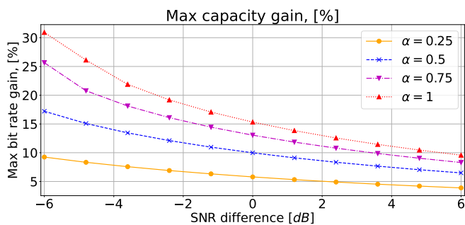
Fig. 10. The maximum achievable capacity gain as a function of the power level difference of neighboring channels compared to the current channel. Negative values indicate that the neighbors are weaker, while positive values indicate that the neighbors are stronger. For the sake of clarity, we assume that both neighbors have the same higher or lower SNR level.
