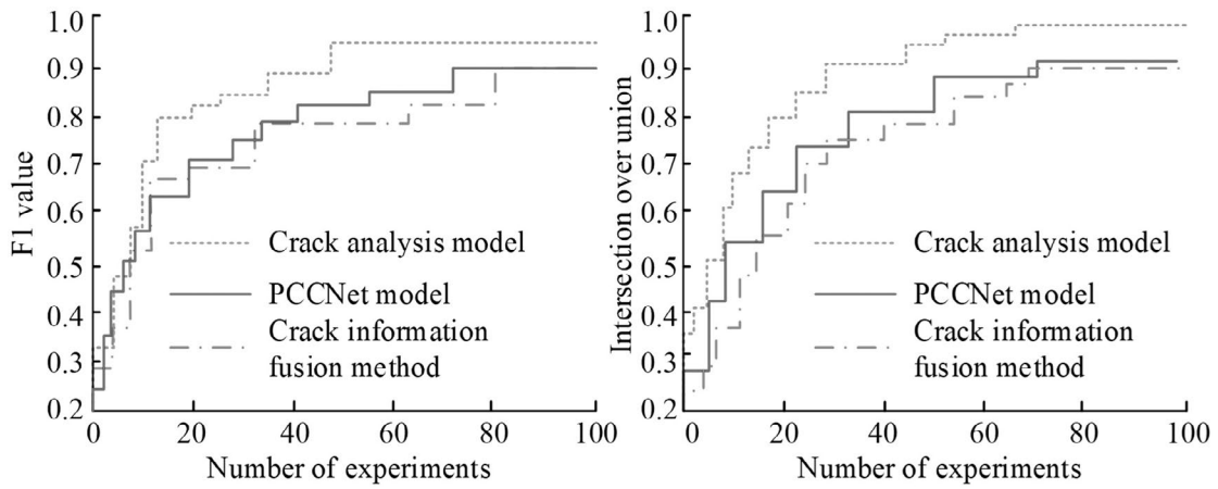
(a) Comparison results of F1 values for three methods. (b) Comparison results of Intersection over Union.
