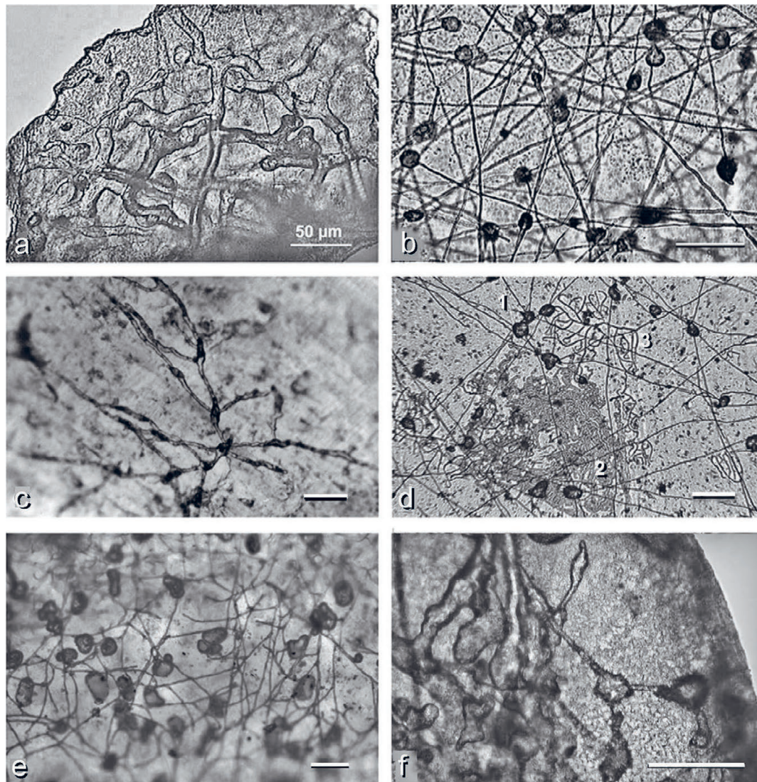
Figure 2. Outlines of various microbial borings in transparent shells from the 1550 m deep Blake Platform – transmitted light micrographs, all scale bars are 50 \mu m long. a. Shell fragment densely bored by Orthogonum isp. b. A network of crisscrossed hyphal tunnels interconnecting sporangial swellings of Saccomorpha . c. Outlines of Saccomorpha guttulata , with ramified sections and spindle-shaped swellings; note dark content indicating residual organism or precipitate. d. A network of Saccomorpha (1) superimposed over the shell surface corroded by Scolecia serrata (2) and S. urbimetra isp. nov. (3). e. Network of Saccomorpha stereodiktyon , with numerous sporangia adhering to the shell's interior surface. f. Saccomorpha guttulata , in a transparent keel of the foraminifera Laticarinina pauperata (PARKER & JONES, 1865) from 1,645 m depth at Bermuda Pedestal, Atlantic Ocean.
