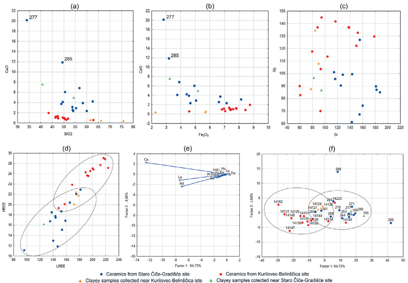
Figure 6. Bivariate plots of (a) SiO 2 vs CaO, (b) Fe 2 O 3 vs CaO, (c) Sr vs Rb, (d) LREE (La, Ce, Pr, Nd, Sm, Eu) vs HREE (Gd, Tb, Dy, Ho, Er, Tm, Yb, Lu), (e) projection of the variables on the factor-plane and (f) principal component analysis based on REE conducted on ceramics from the Staro Čiče-Gradišće and Kurilovec-Belinščica site and on clayey samples.
