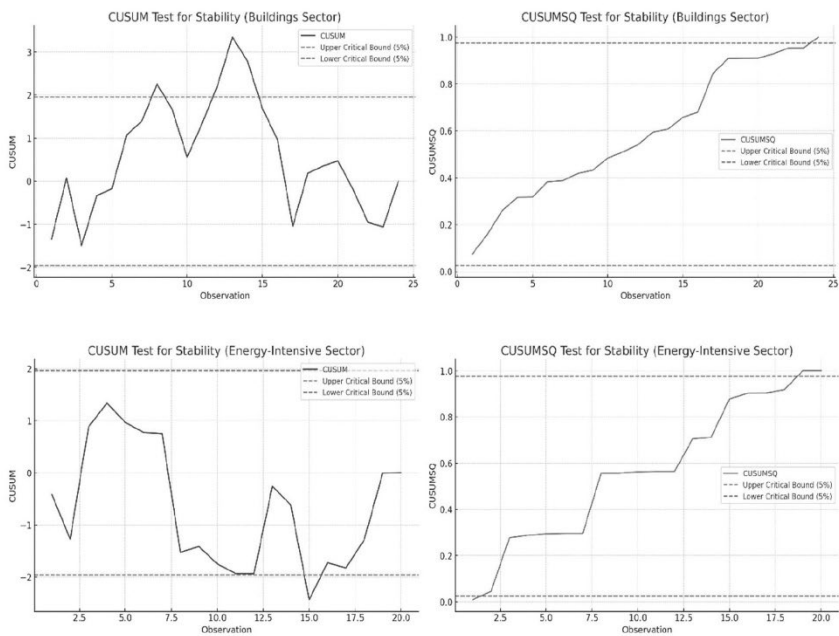
Figure A1 CUSUM and CUSUMSQ test results
