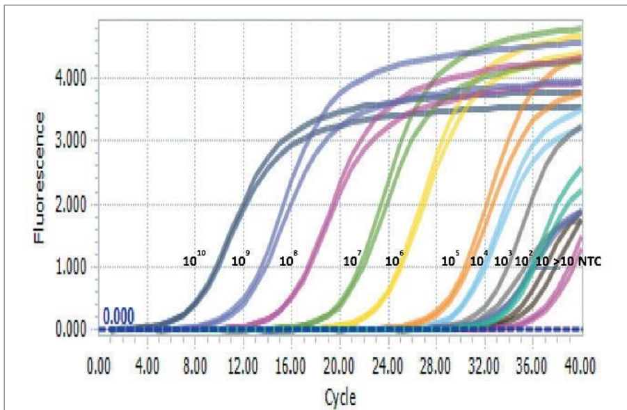
Fig. 2. Amplification plot detection of the 590bp hexon gene by SYBR Green based real time PCR
