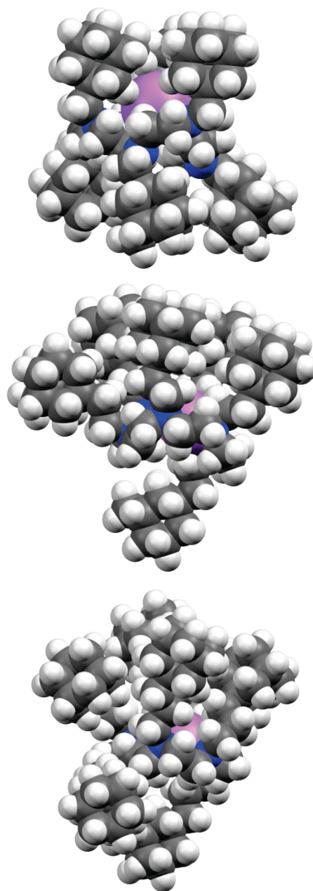
Figure 2. Optimized structures of sodium complexes with hosts 1–3 , from top to bottom: 1 ·Na + , 2 ·Na + , and 3 ·Na + .
