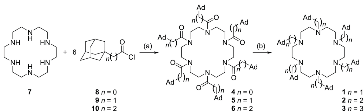
Scheme 1. Preparation of hexaadamantyl hexaaza crown ethers 1–3 . (a) DMA, DMAP, Et 3 N, CH 2 Cl 2 , (b) LiAlH 4 , Et 2 O.
