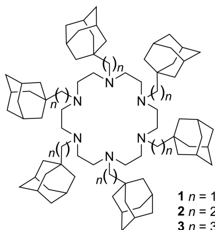
Figure 1. Structures of hexaaza crown ethers 1–3 substituted with six adamantyl subunits.
