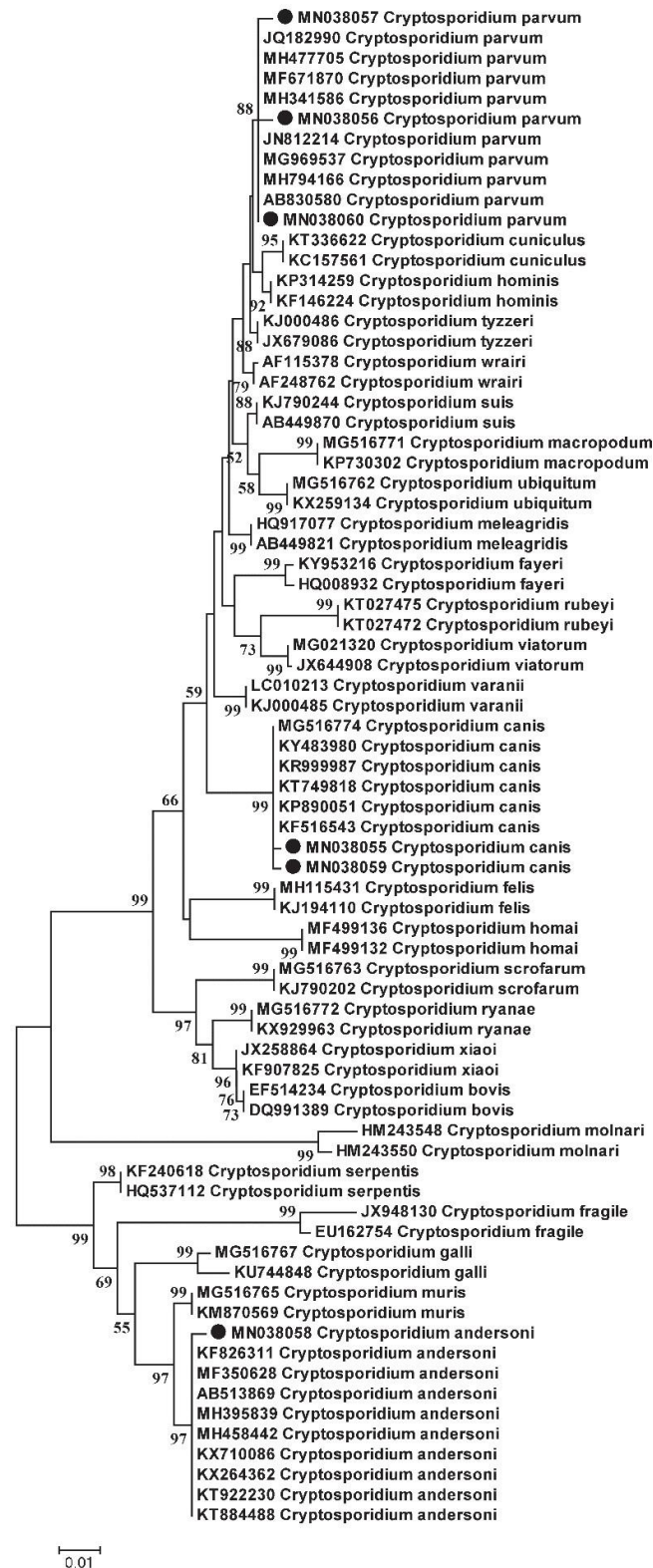
Fig. 2. Phylogenetic analysis of Cryptosporidium spp. based on sequences of the partial 18S ribosomal RNA gene
