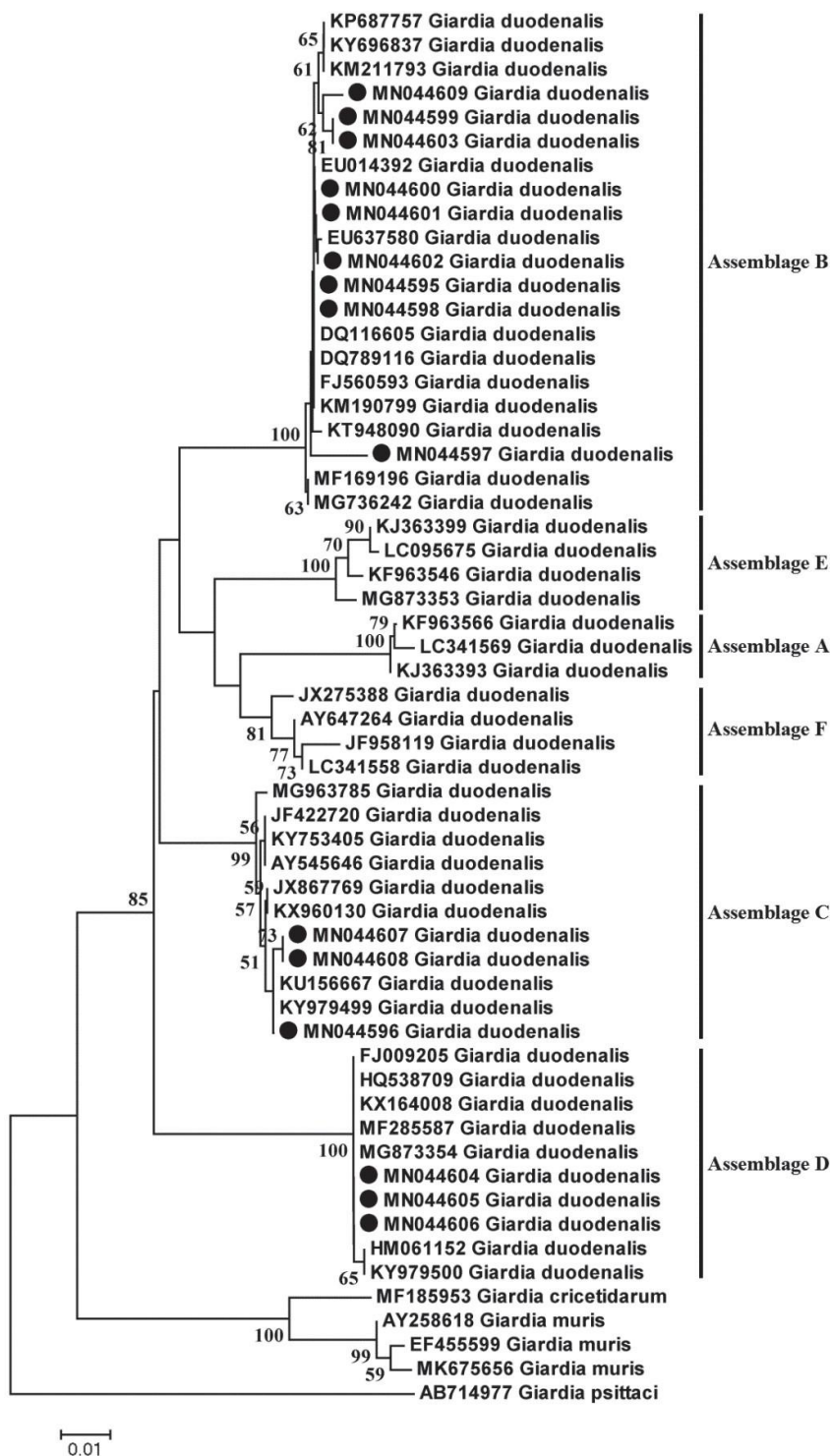
Fig. 3. Phylogenetic analysis of Giardia based on sequences of the partial \beta -giardin gene The black circles represent the positive samples and the assemblages of G. duodenalis identified
