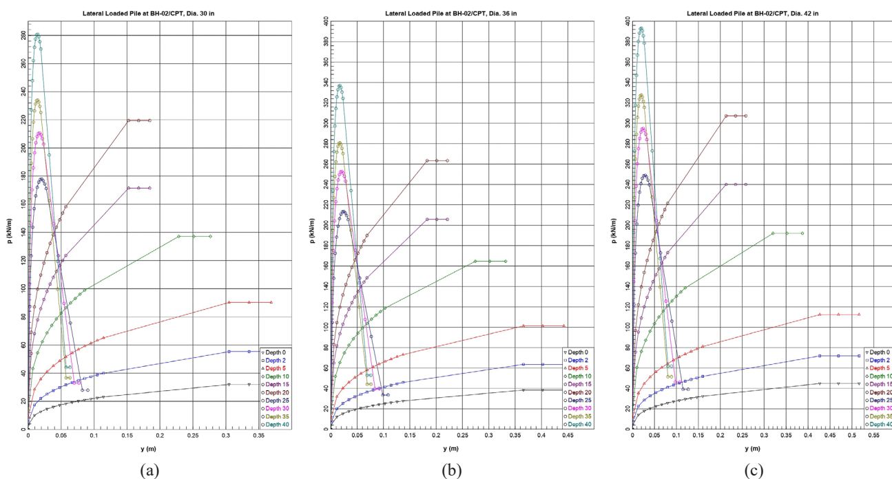
Figure 13: Laterally loaded pile at bh-02/CPT; (a): diameter 0.762 m; (b): diameter 0.914 m; (c): diameter 1.067 m.
