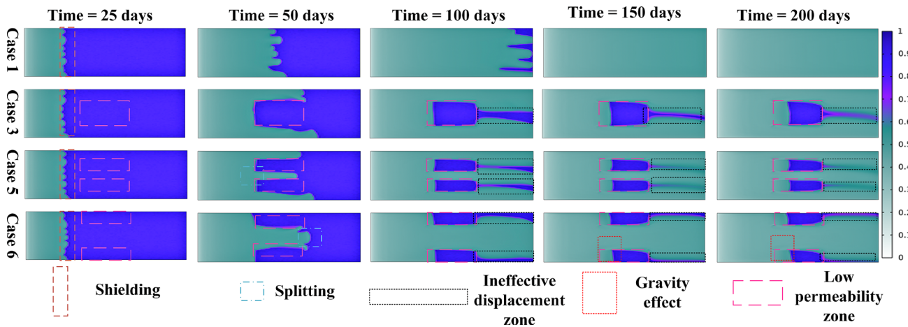
Figure 5: The schematic represents the spatial changes in oil saturation with time enhancement with the low permeability barrier present vertically.
