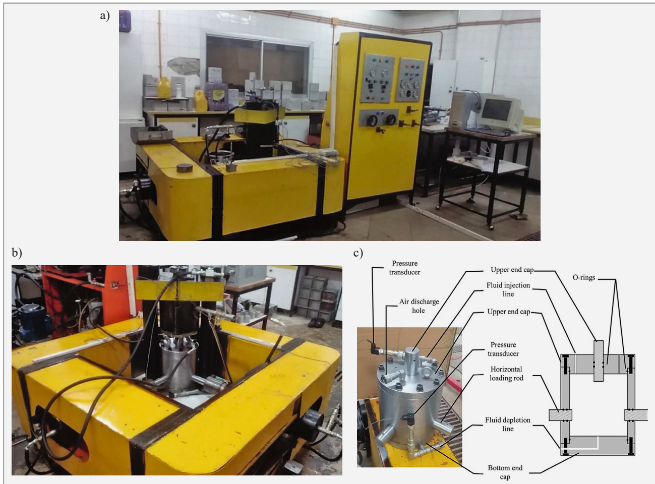
Figure 1: a) Overview of experimental setup; b) The frame and jack for applying axial pressure; c) Pore pressure cell developed to apply injection load on samples (Mortazavi and Atapour, 2018).
