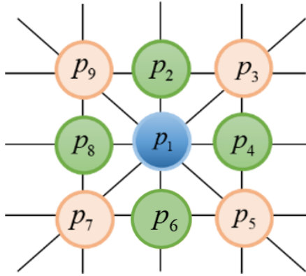
Fig. 1. 3 \times 3 mask for Zhang-Suen algorithm
