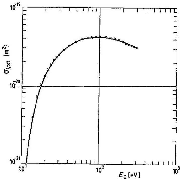
Fig. 1. Total ionization cross section of the methanol molecule by electron impact.
