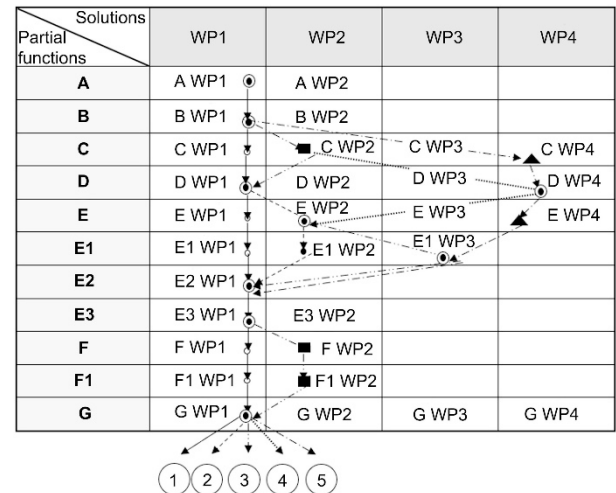
Figure 10 Combinations of working principles that generate variant solutions of a mobile machine for corn peeling
