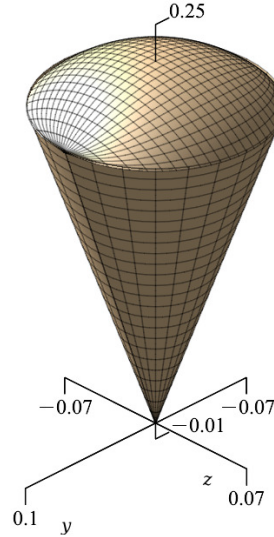
FIGURE 1. a spherical cone in 3 dimensions with central vector (1, 0, 0)
