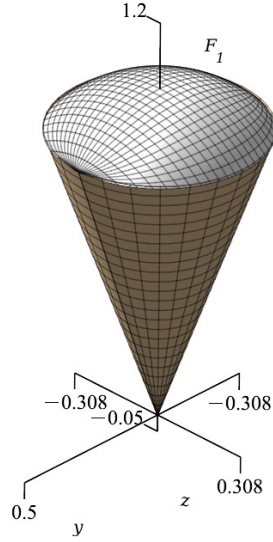
FIGURE 2. a plot of the set F_1 (white color), for the central vector (1, 0, 0) .
