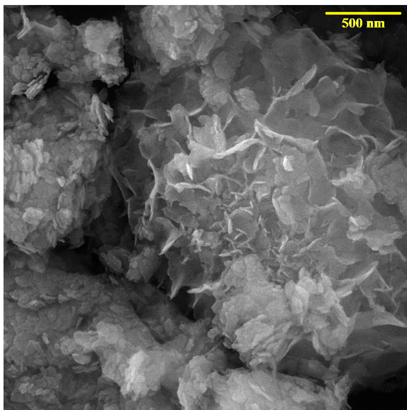
Figure 1. SEM image of NiMoO 4 nanosheets
