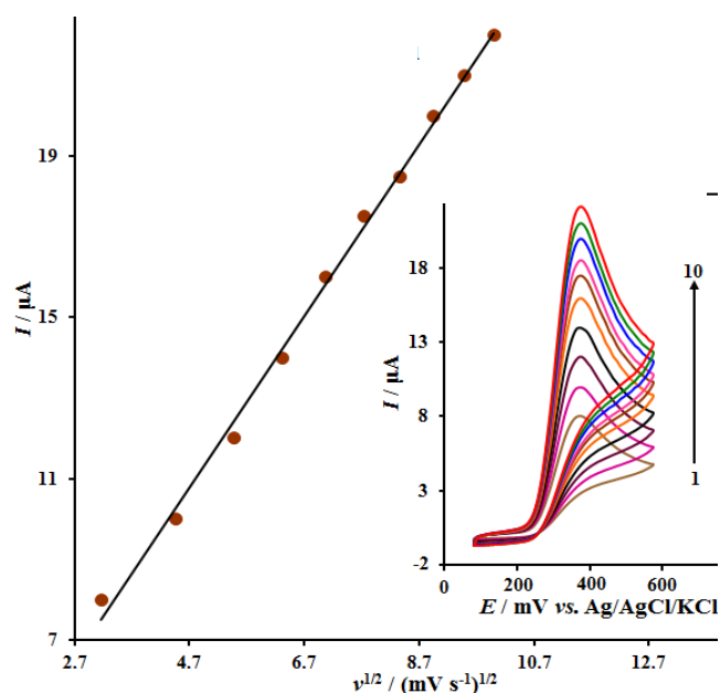
Figure 3. CV responses and the linear response of the I_{pa} with v^{1/2} of the NMs/IL/CPE in the measurement of 100.0 \mu\text{M} epinine in PBS by varying the scan rates. Inset: CVs recorded at (1 to 10): 10, 20, 30, 40, 50, 60, 70, 80, 90 and 100 \text{mV s}^{-1}
