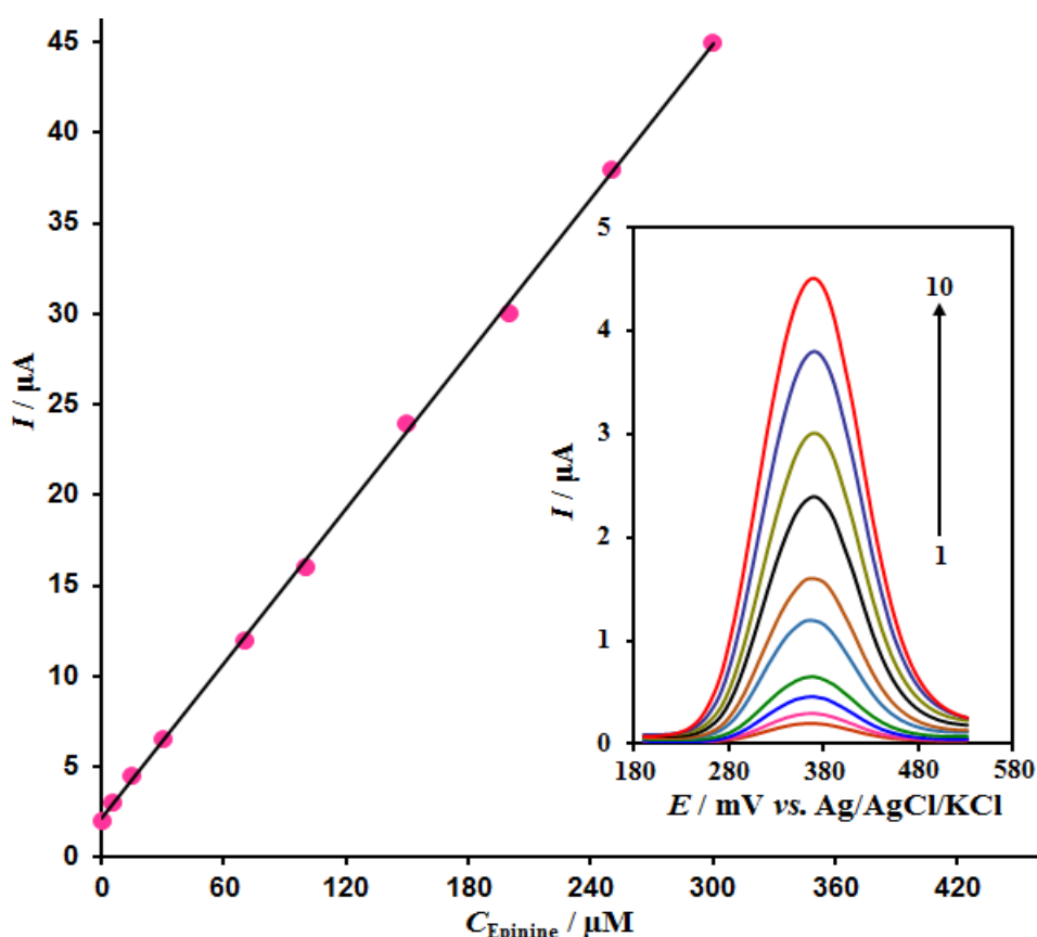
Figure 5. DPV responses and calibration graph for epinine at NMs/IL/CPE in PBS containing diverse concentrations of epinine. Inset: voltammograms 1 to 10 correspond to 0.1, 5.0, 15, 30.0, 70.0, 100.0, 150.0, 200.0, 250.0 and 300.0 \mu\text{M} of epinine
