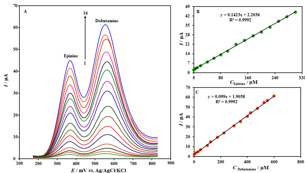
Figure 6. A -DPV responses of NMs/IL/CPE (voltammograms 1 to 16 correspond to 0.1 + 1.0, 5.0 + 10.0, 10.0 + 30.0, 20.0 + 50.0, 40.0 + 100.0, 60.0 + 125.0, 80.0 + 175.0, 100.0 + 225.0, 125.0 + 300.0, 150.0 + 350.0, 175.0 + 400.0, 200.0 + 425.0, 225.0 + 475.0, 250.0 + 525.0, 275.0 + 550.0 and 300.0 + 600.0 \mu\text{M} epinine and dobutamine, respectively) and calibration graphs for B- epinine and C -dobutamine in PBS containing diverse concentrations of epinine and dobutamine
