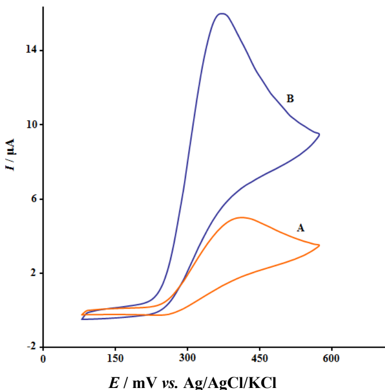
Figure 2. CVs of unmodified CPE (A) and NMs/IL/CPE (B) in PBS containing epinine (100.0 \mu\text{M} )
