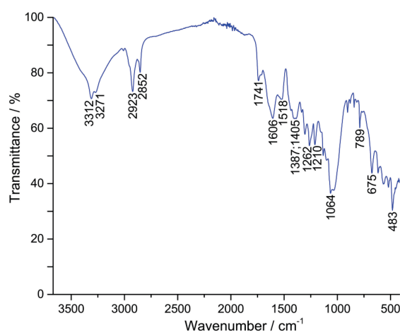
Figure 4. ATR-IR spectrum of Cabernet Franc 2020.
