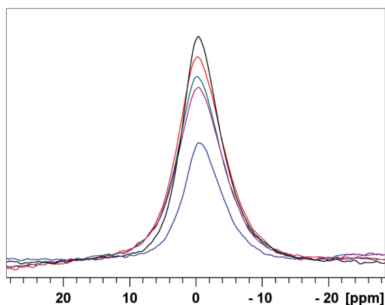
Figure 2. ^{31}\text{P} MAS NMR spectra of the GP samples. From top to bottom: Cabernet Franc 2020, Merlot 2020, Cabernet Sauvignon 2020, Cabernet Sauvignon 2017, Plavac Mali 2024.
