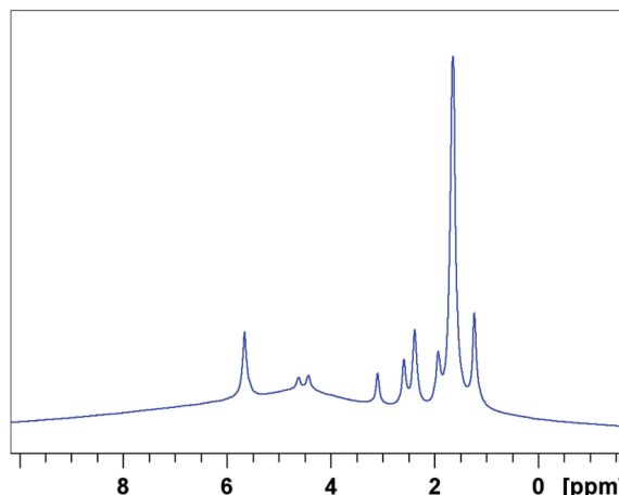
Figure 3. Representative ^1\text{H} MAS spectrum of Cabernet Franc 2020.
