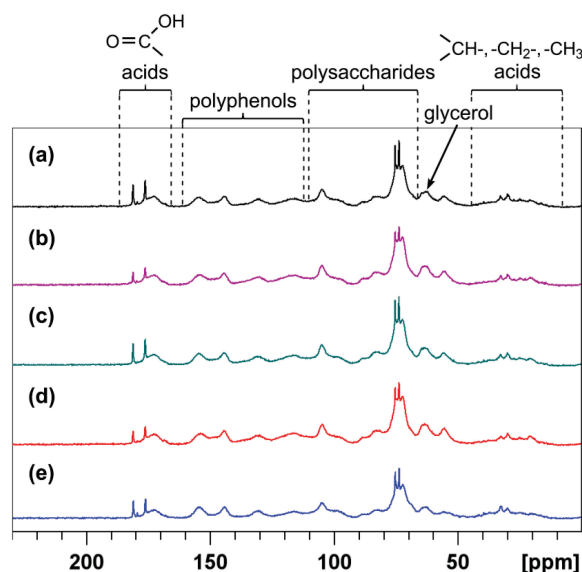
Figure 1. ^{13}\text{C} CP MAS NMR spectra of the GP samples: (a) Cabernet Franc 2020, (b) Cabernet Sauvignon 2017, (c) Cabernet Sauvignon 2020, (d) Merlot 2020 and (e) Plavac Mali 2024.
