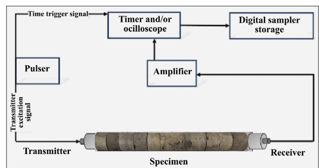
Figure 3. A simplified diagram illustrating the fundamental elements of an ultrasonic apparatus. This study transformed a group of rock cores into jointed rock samples with a total sample length ranging from 0.3 to 1 m. The cores were cut perpendicular to their axis to create artificial joints using a rock cutter to form parallel joints.
