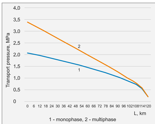
Figure 2. Change in pressure in the gas pipeline (D= 0.2m)
