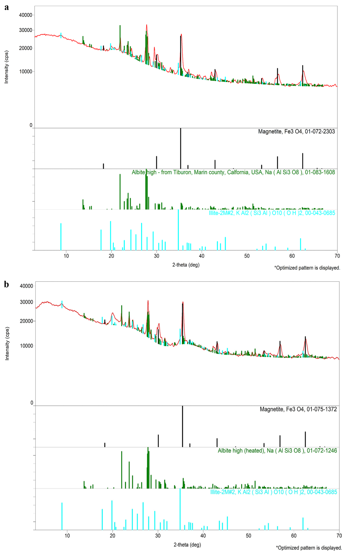
Figure 7. XRD measurement results for study at Ranu Klakah: a) R6 (representative sample from lake – near outlet); b) U2 (representative sample from spring).
