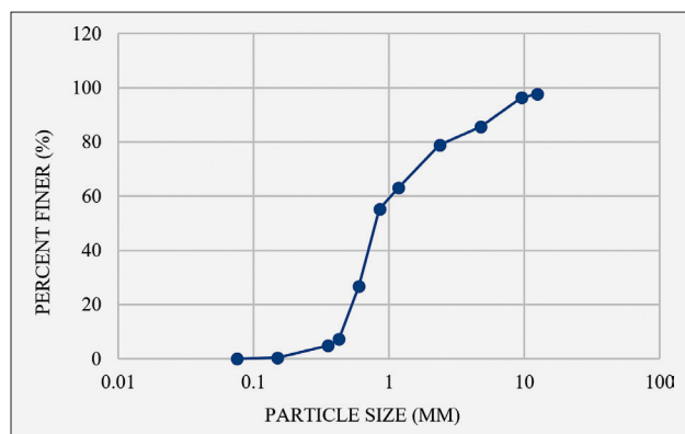
Figure 3. Soil gradation chart used in grout penetration test
