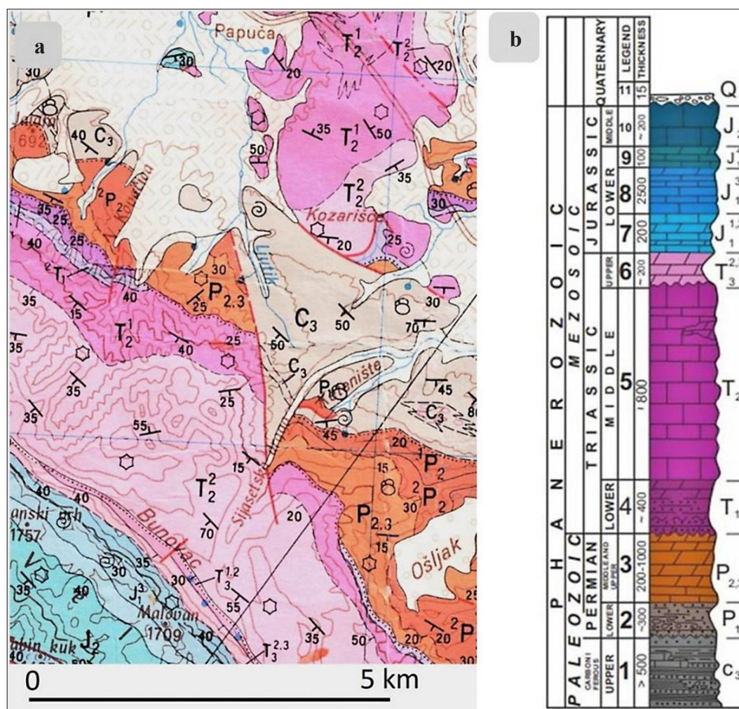
Figure 4. a) fragment from the Basic Geological Map, sheet Udbina (Šušnjarić et al., 1973). Map symbols: C 3 = Upper Carboniferous sandstones and shales; 2 P 2 = Middle Permian sandstones; P 2,3 = Middle and Upper Permian dolomites; T 1 = Lower Triassic dolomites, micaceous sandstones and shales; 2 T 1 = Lower Triassic limestones, marls and dolomites; T 1 1 = Middle Triassic (Anisian) dolomites; T 2 2 = Middle Triassic (Ladinian) limestones and dolomites; T 1,2 1,2 = Upper Triassic conglomerates and tuffaceous clastic deposits; T 2,3 2,3 = Upper Triassic dolomites and limestones; J 1,2 1,2 = Lower Jurassic limestones and dolomites; J 3 3 = Lower Jurassic limestones; J 4 4 = Lower Jurassic spotty limestones; J 2 2 = Middle Jurassic limestones and dolomites; pr = proluvial gravels and sands b) Stratigraphic column of the area Vaganski Vrh-Papuča.
