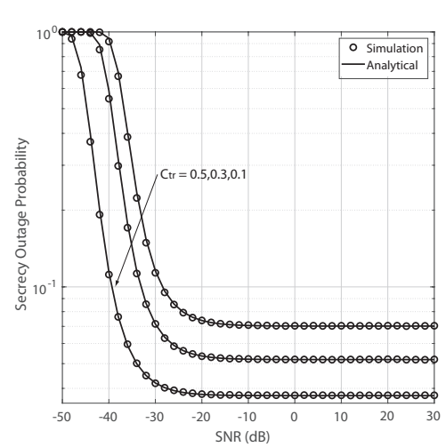
Fig. 14. SOP versus SNR for different values of C_{tr} for active IRS based system
