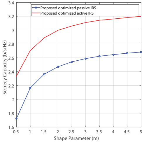
Fig. 7. Secrecy capacity versus Nakagami shape parameter m for proposed optimized passive and active IRS with N = 6
