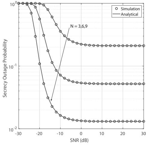
Fig. 9. SOP versus SNR for different values of N for the proposed optimized passive IRS-assisted system
