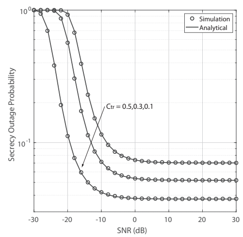
Fig. 13. SOP versus SNR for different values of C_{tr} for passive IRS based system
