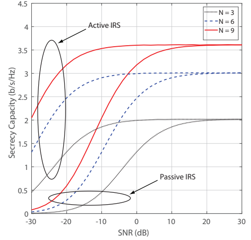
Fig. 4. Secrecy capacity versus SNR for proposed optimized passive and active IRS for different values of N
