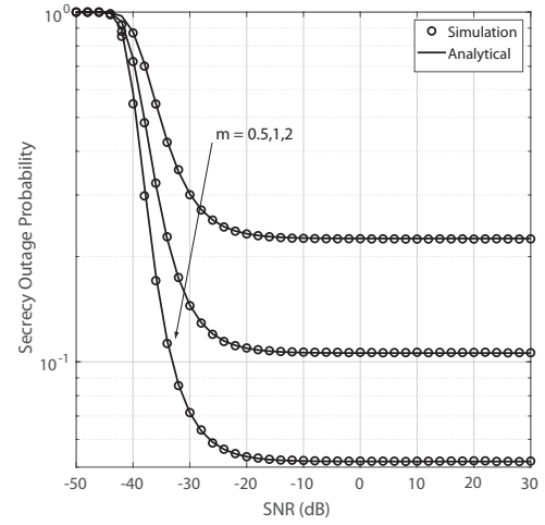
Fig. 12. SOP versus SNR for different values of m for the proposed optimized active IRS-based system
