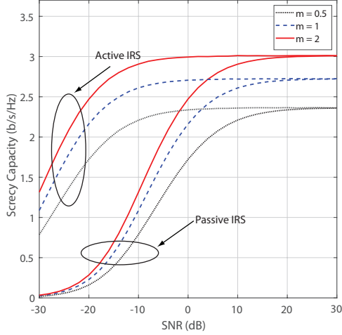
Fig. 6. Secrecy capacity versus SNR for proposed optimized passive and active IRS for different values of Nakagami shape parameter m with N = 6
