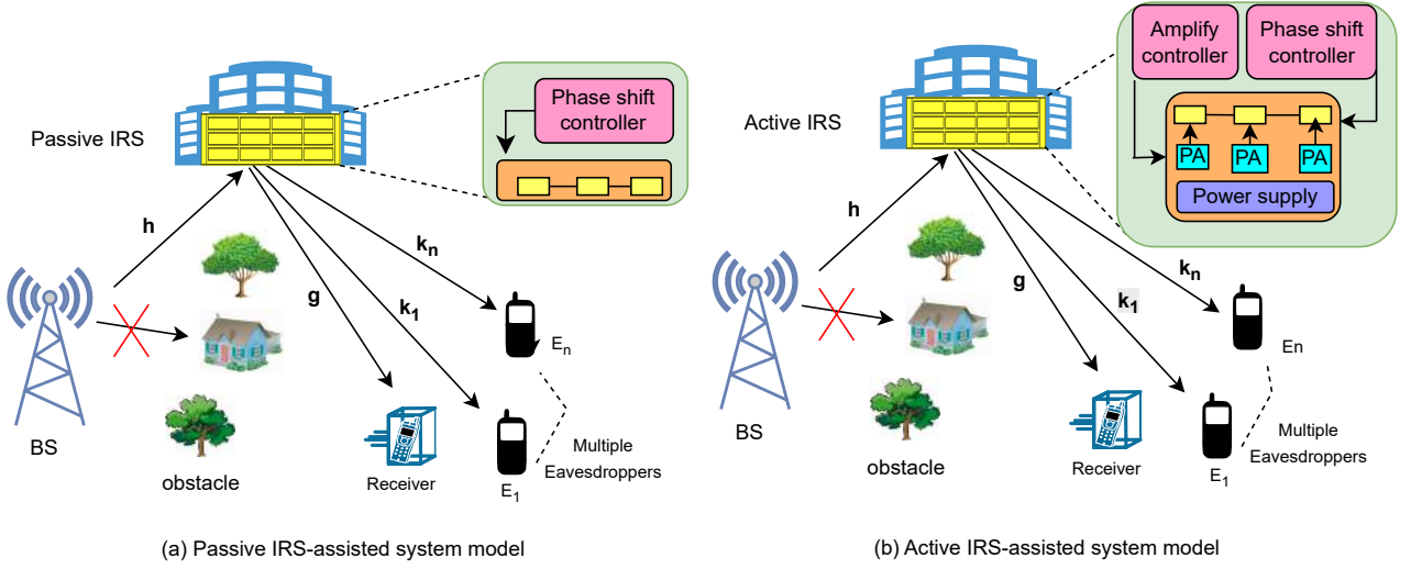
Fig. 2. Proposed passive and active IRS-based communication system model
