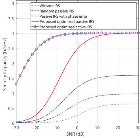
Fig. 3. Secrecy capacity versus SNR for different schemes with single eavesdropper and N = 6
