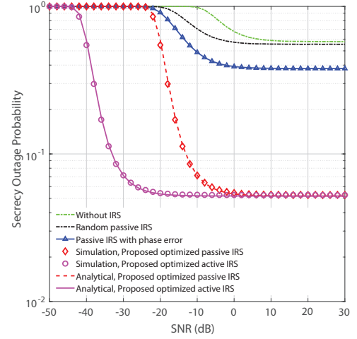
Fig. 8. SOP versus SNR for different schemes with single eavesdropper and N = 6
