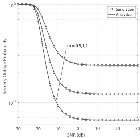
Fig. 11. SOP versus SNR for different values of m for the proposed optimized passive IRS based system
