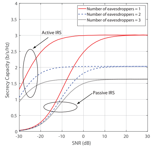
Fig. 5. Secrecy capacity versus SNR for proposed optimized passive and active IRS for different number of eavesdroppers with N = 6
