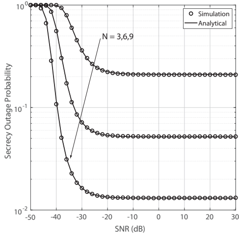
Fig. 10. SOP versus SNR for different values of N for the proposed optimized active IRS based system
