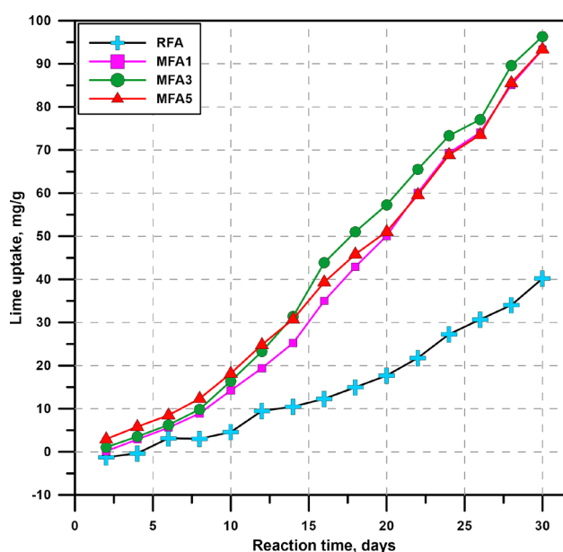
Figure 7. Lime uptake of the RFA and MFAs
