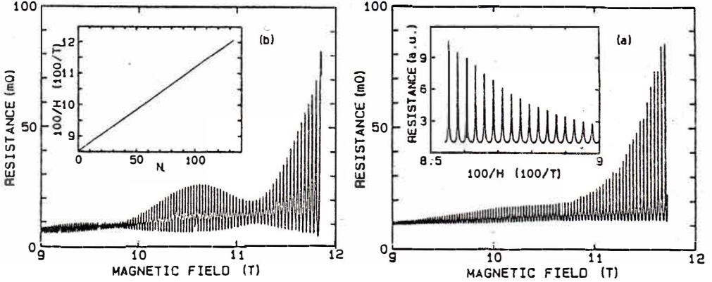
Fig.4: Magnetoresistance of \beta_{\text{H}}\text{-(ET)}_2\text{I}_3 between 9 and 12 T at 0.38 K and 1/H plot of the peak positions versus integer numbers (left inset). The oscillations become strongly anharmonic at highfields (right inset).
