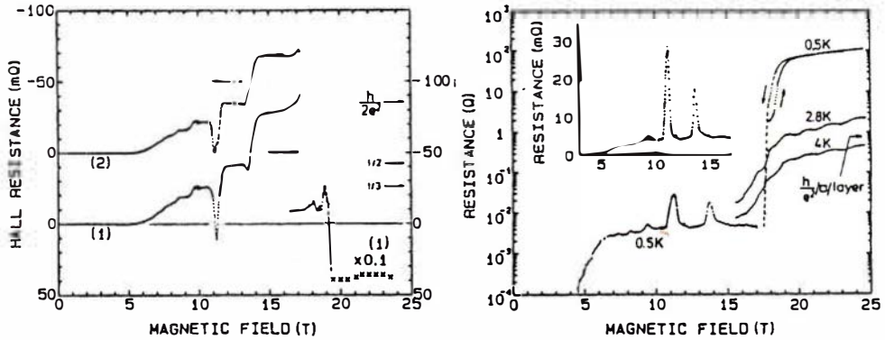
Fig.3: Hall resistance versus magnetic field along the c^* axis for two (\text{TMTSF})_2\text{PF}_6 samples ( P \approx 9 kbar, T = 0.5 K). The quantized values h/2ne^2 = 12.9/n \text{k}\Omega per molecular layer are marked on the right for sample #1. The n = 0 phase is reached above 18 T (left). Magnetoresistance of the same sample up to 25T (linear scale in the inset).
