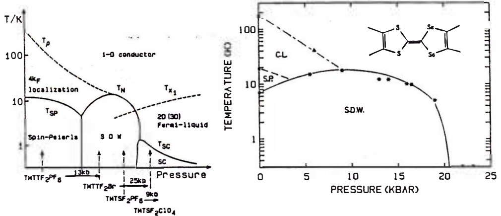
Fig.1: Generalized phase diagram of (TMTCF)_2X conductors (left) and phase diagram of (TMDTDSF)_2PF_6 showing the reentrance of SDW below the spin-Peierls state at 7 K and the stabilization of a conducting ground state above 20 kbar (without superconductivity down to 0.4K).
