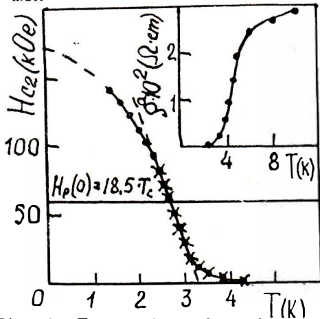
Fig. 1: Temperature dependences of upper critical fields H_{C2}^a and H_{C2}^{b'} parallel to the ab plane of the (\text{BEDT-TTF})_4\text{Hg}_{2.89}\text{Br}_8 single crystal. ( \bullet ) H_{C2}^a ; ( \times ) H_{C2}^{b'} . The inset illustrates the resistivity vs. temperature plot at H=0 .
