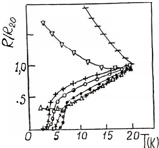
Fig. 3: Temperature dependence of resistivity of the single crystals (\text{BEDT-TTF})_4\text{Hg}_{2.89}\text{Br}_8 at various pressures.
