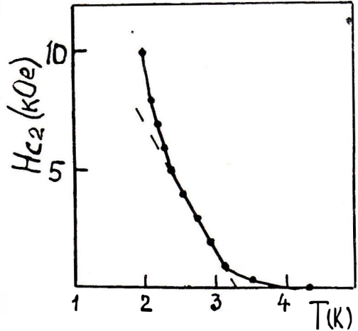
Fig. 2: Temperature dependence of the upper critical field H_{C2}^{c*} perpendicular to the ab plane, H_{C2}^{c*} .
